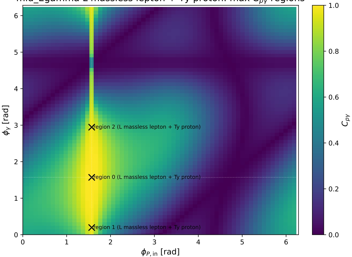
mid_Egamma L massless lepton + Ty proton: max C_{p\gamma} regions
