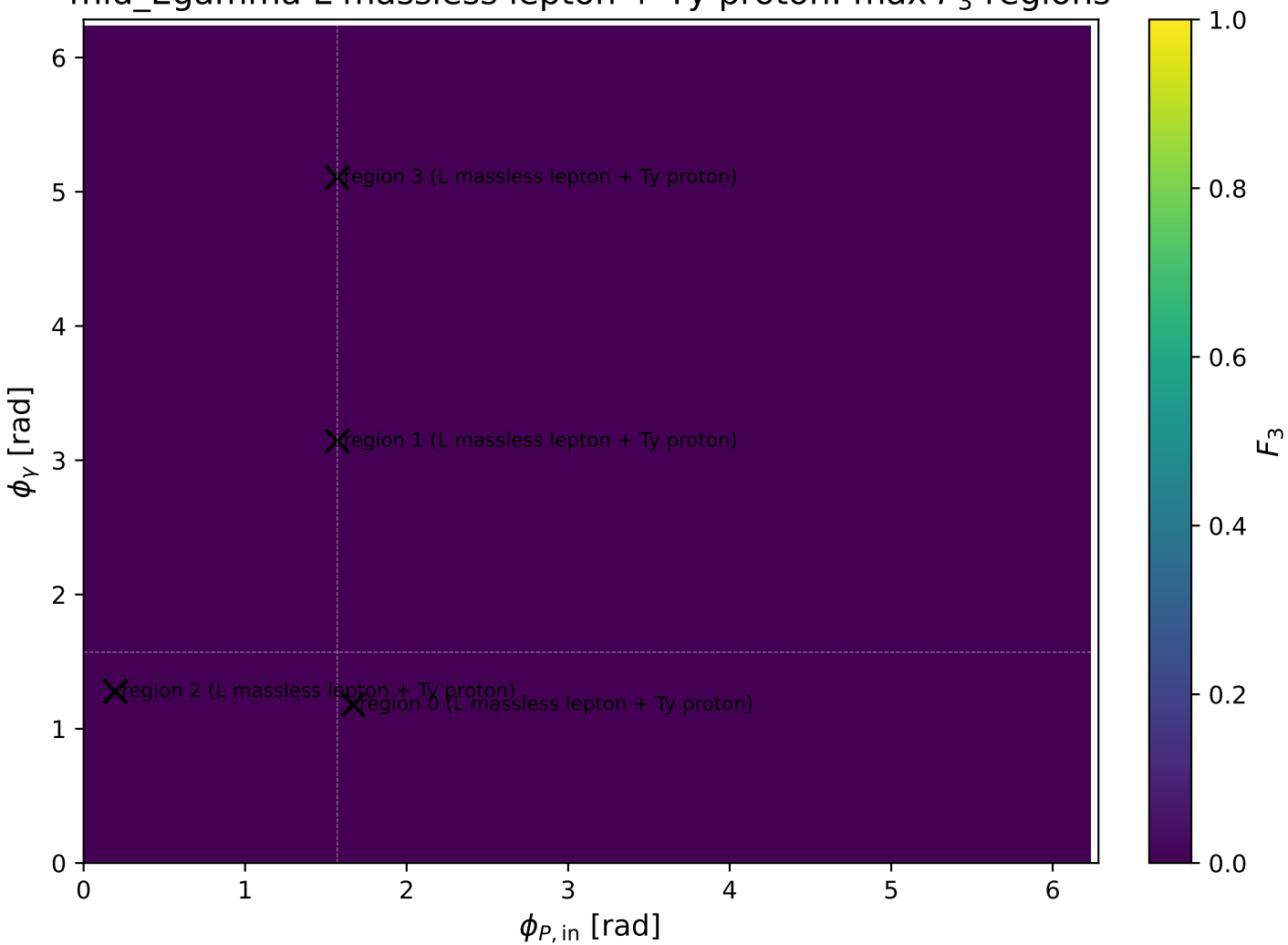
mid_Egamma L massless lepton + Ty proton: max F_3 regions
