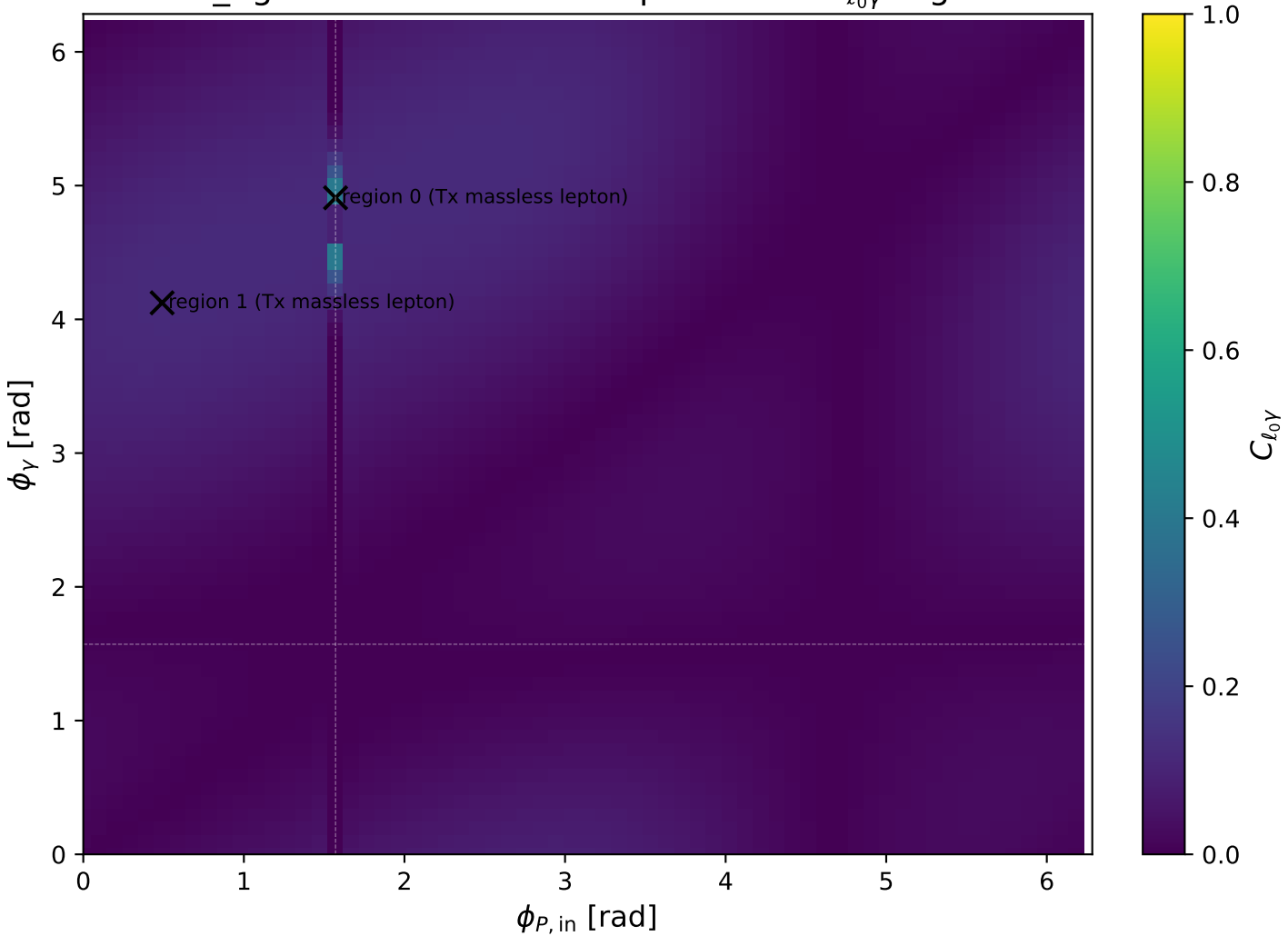
low_Egamma Tx massless lepton: max C_{\ell_0\gamma} regions
