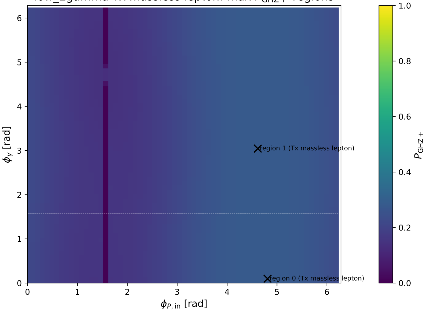
low_Egamma Tx massless lepton: max P_{\text{GHz}+} regions
