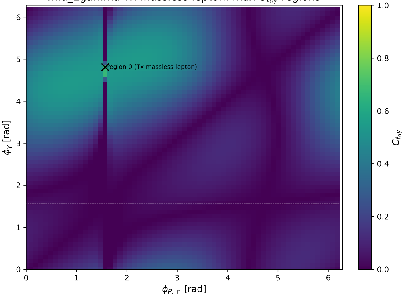
mid_Egamma Tx massless lepton: max C_{\ell_0\gamma} regions
