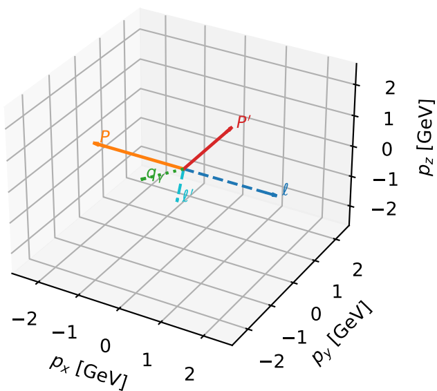
3D momenta
