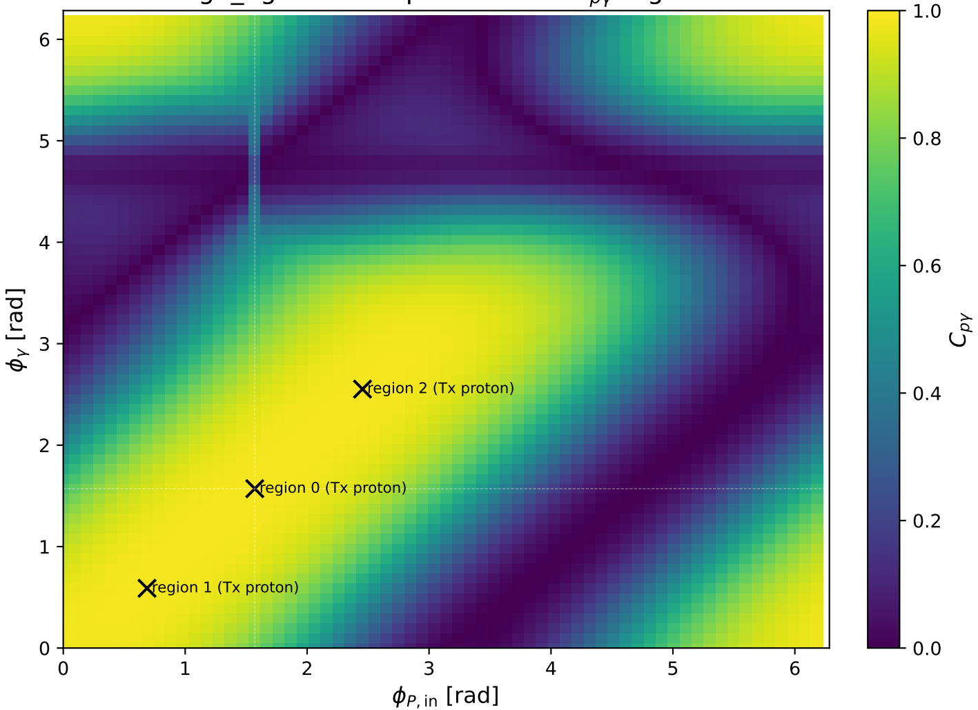
high_Egamma Tx proton: max C_{p\gamma} regions
