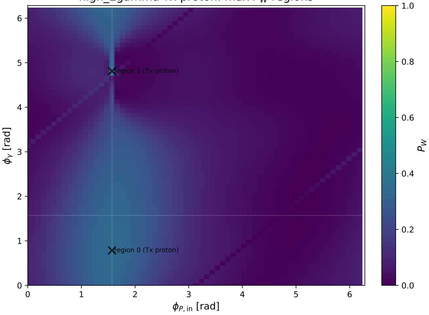
high_Egamma Tx proton: max P_W regions
