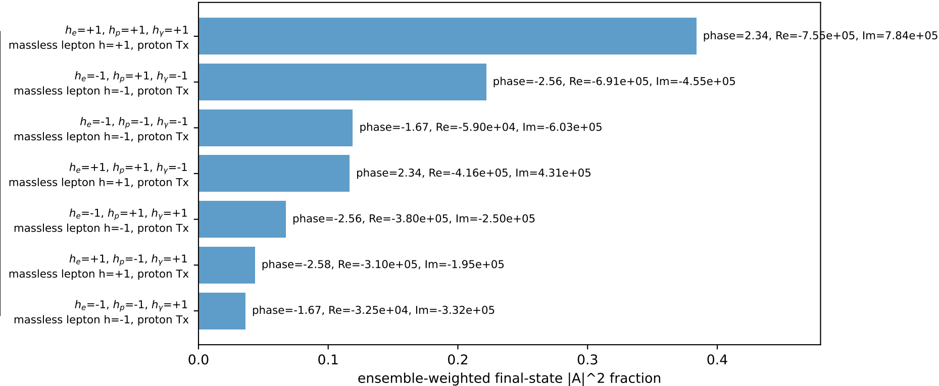
Leading initial-ensemble/final-state components (N=7, retained=98.7%)
