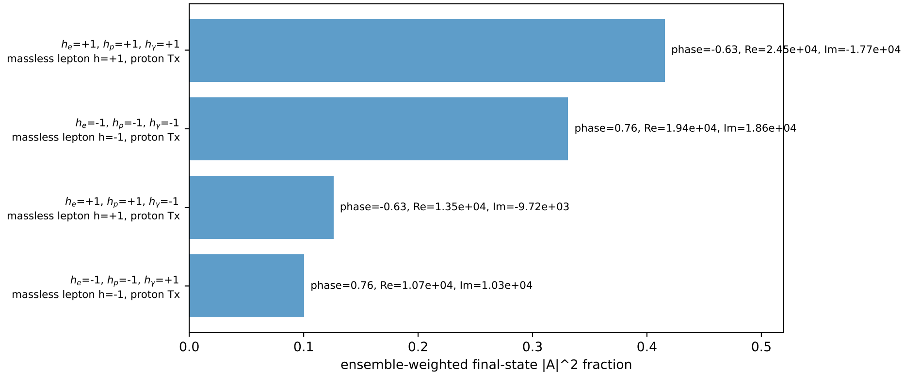
Leading initial-ensemble/final-state components (N=4, retained=97.3%)
