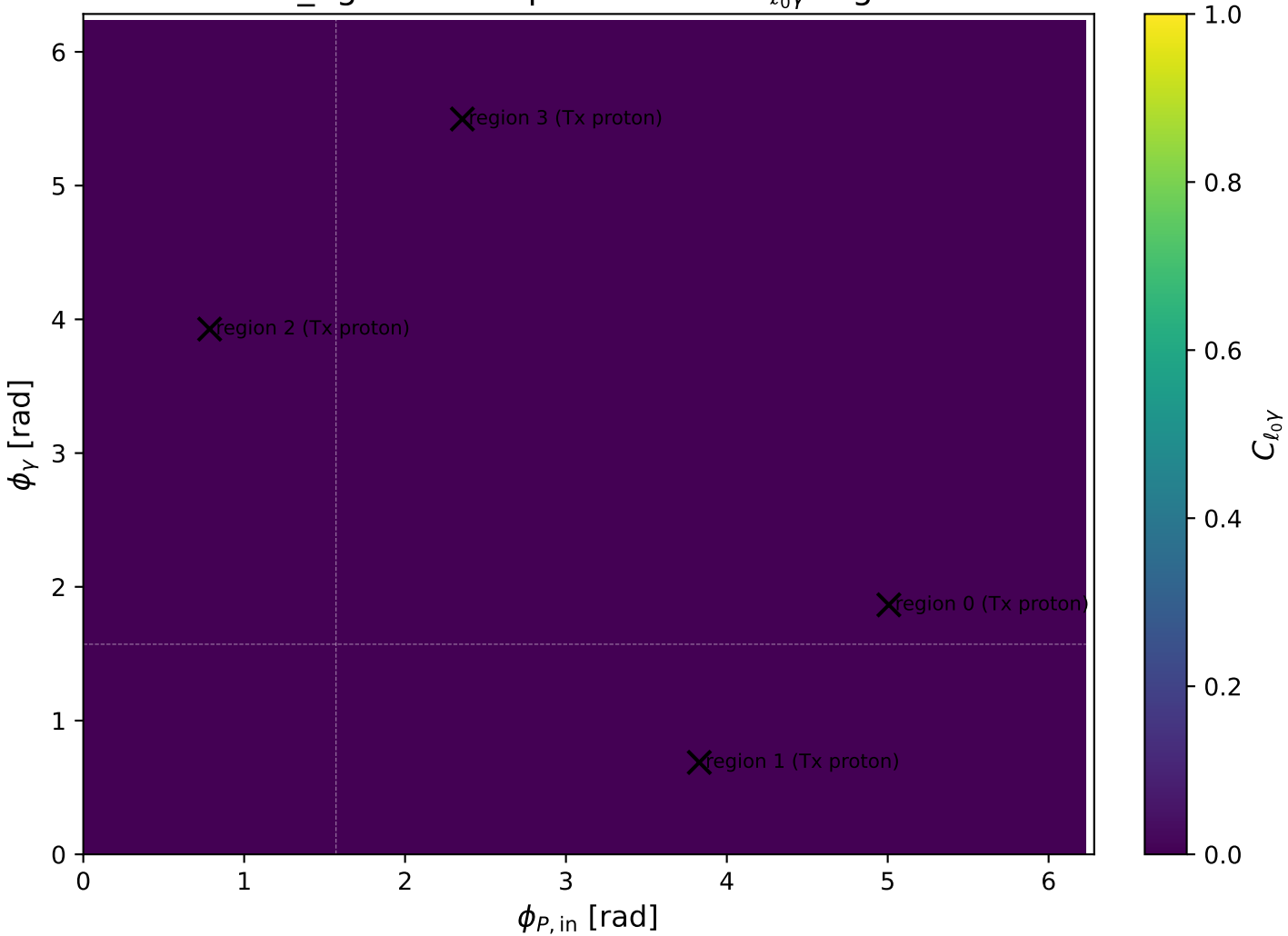
mid_Egamma Tx proton: max C_{\ell_0\gamma} regions
