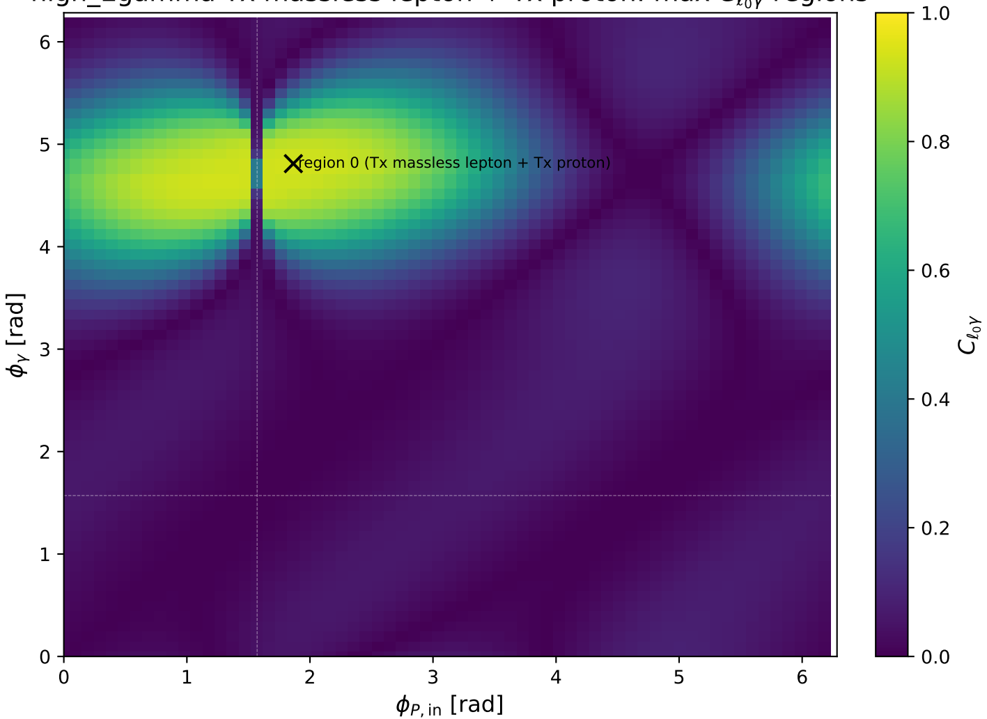
high_Egamma Tx massless lepton + Tx proton: max C_{\ell_0\gamma} regions
