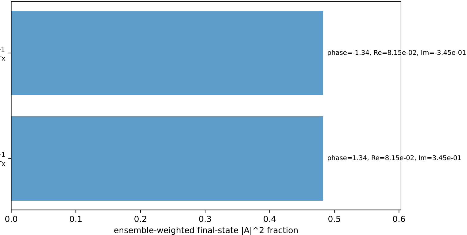
Leading initial-ensemble/final-state components (N=2, retained=96.5%)
