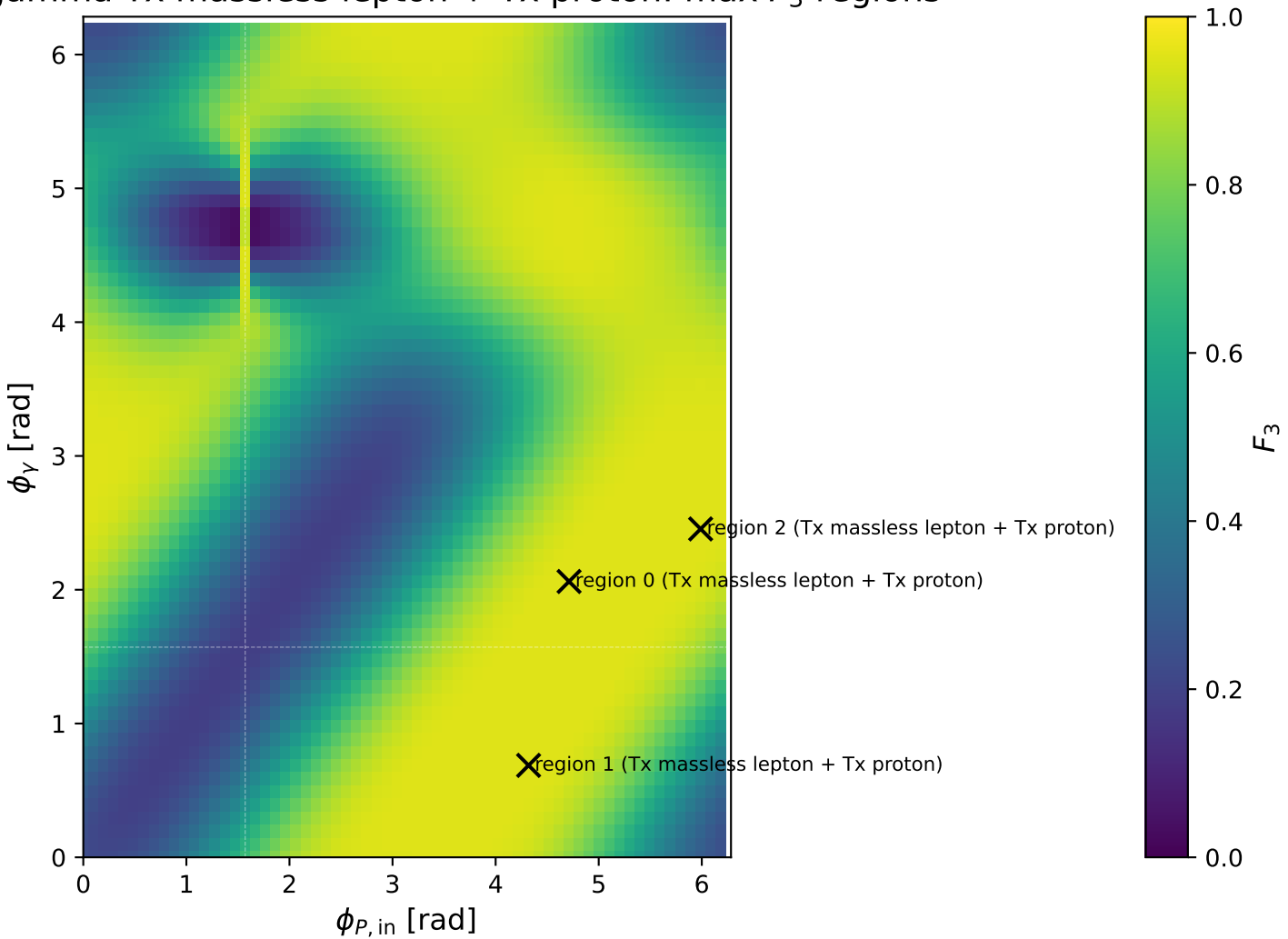
gamma Tx massless lepton + Tx proton: max F_3 regions
