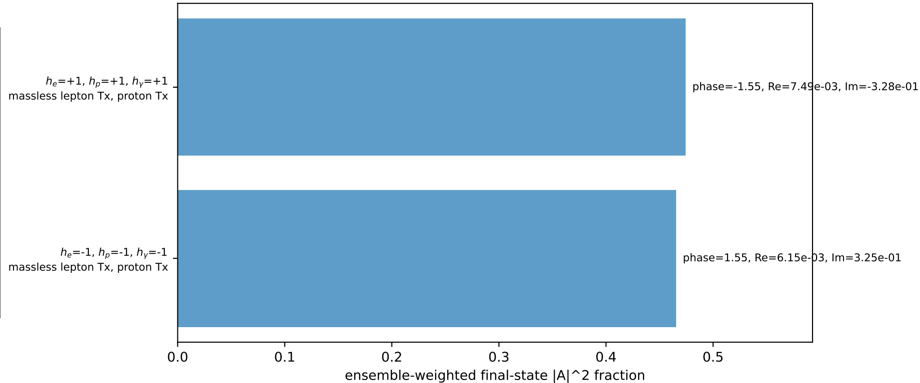
Leading initial-ensemble/final-state components (N=2, retained=94.0%)
