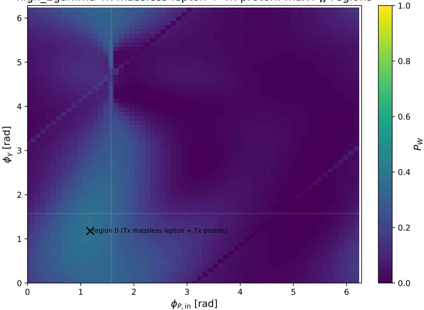
high_Egamma Tx massless lepton + Tx proton: max P_W regions
