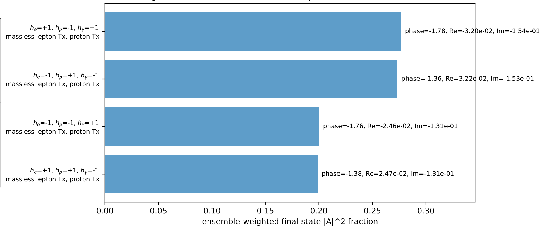
Leading initial-ensemble/final-state components (N=4, retained=94.9%)
