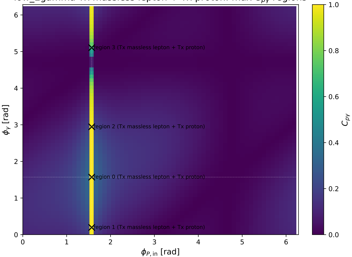
low_Egamma Tx massless lepton + Tx proton: max C_{py} regions
