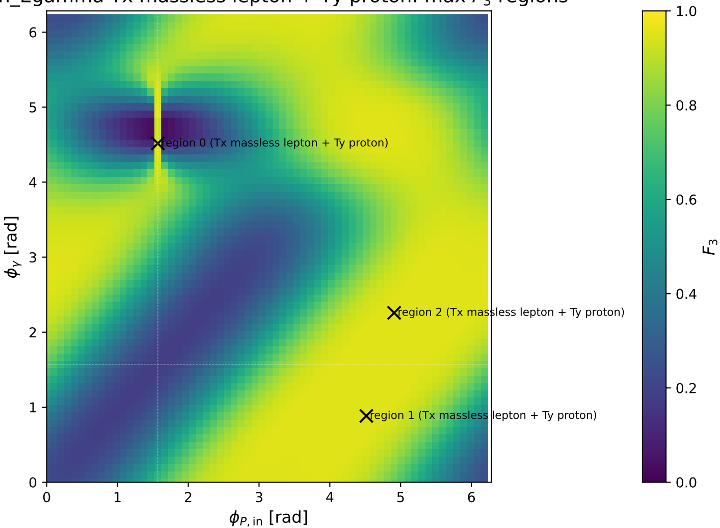
h_Egamma Tx massless lepton + Ty proton: max F_3 regions
