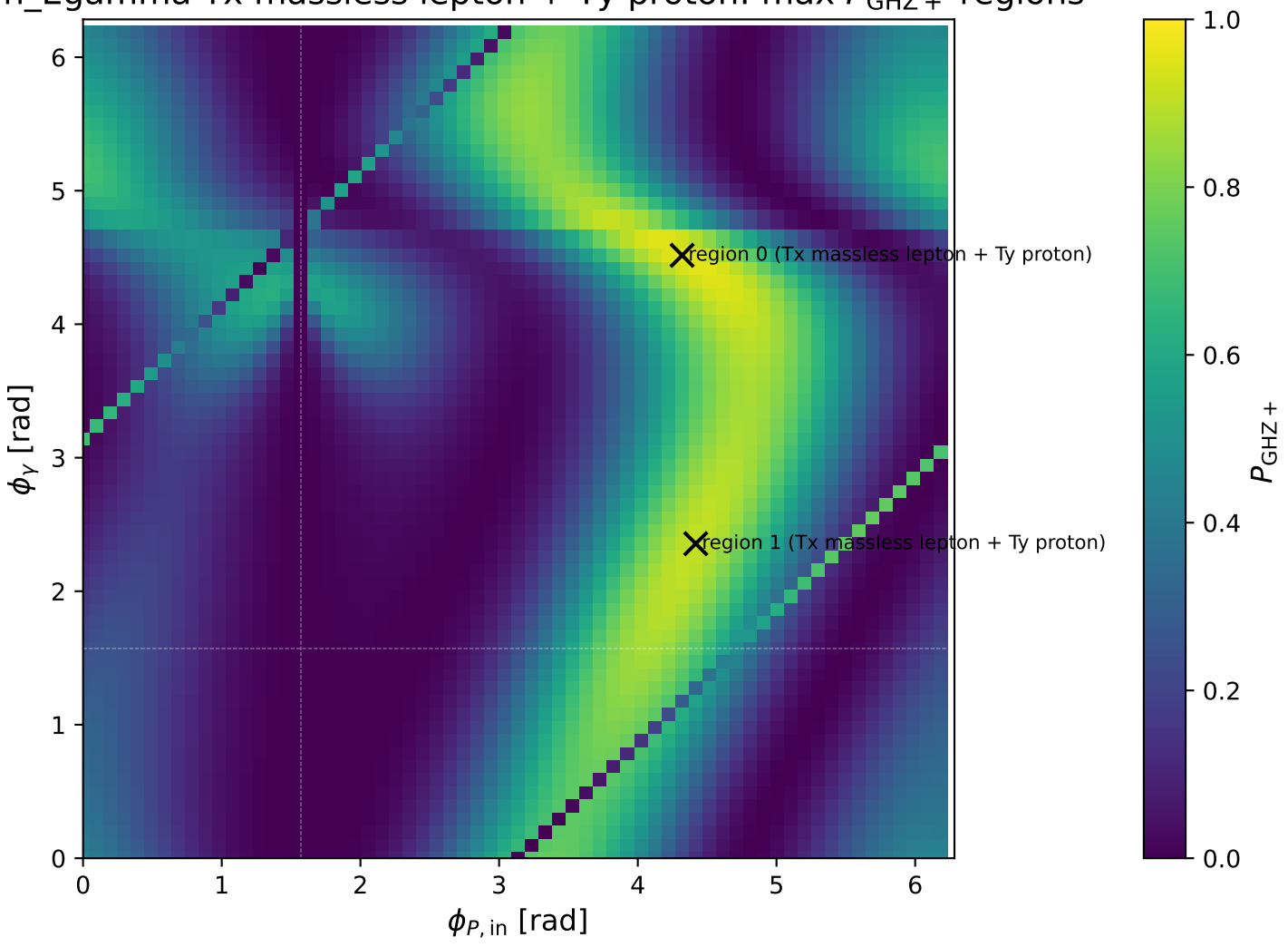
h_Egamma Tx massless lepton + Ty proton: max P_{\text{GHZ}} + regions
