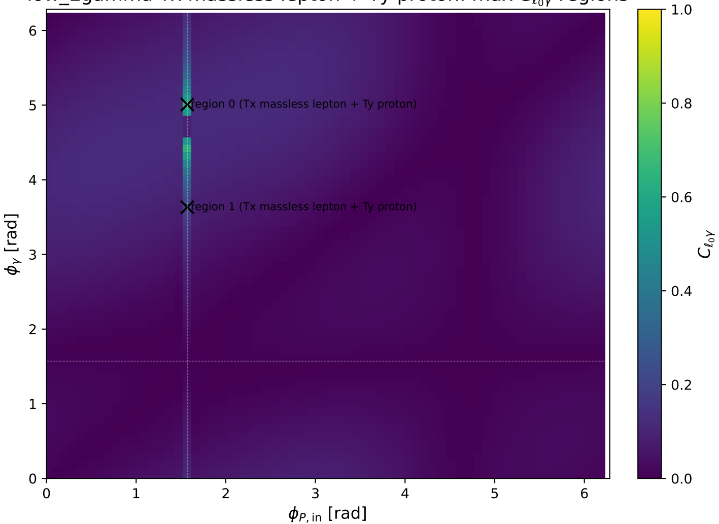
low_Egamma Tx massless lepton + Ty proton: max C_{\ell_0\gamma} regions
