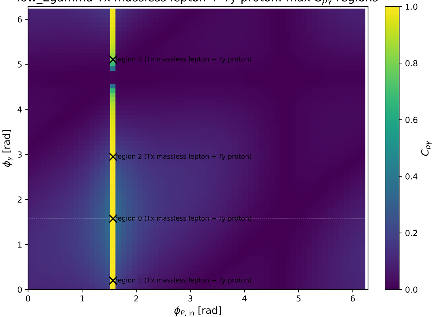
low_Egamma Tx massless lepton + Ty proton: max C_{p\gamma} regions
