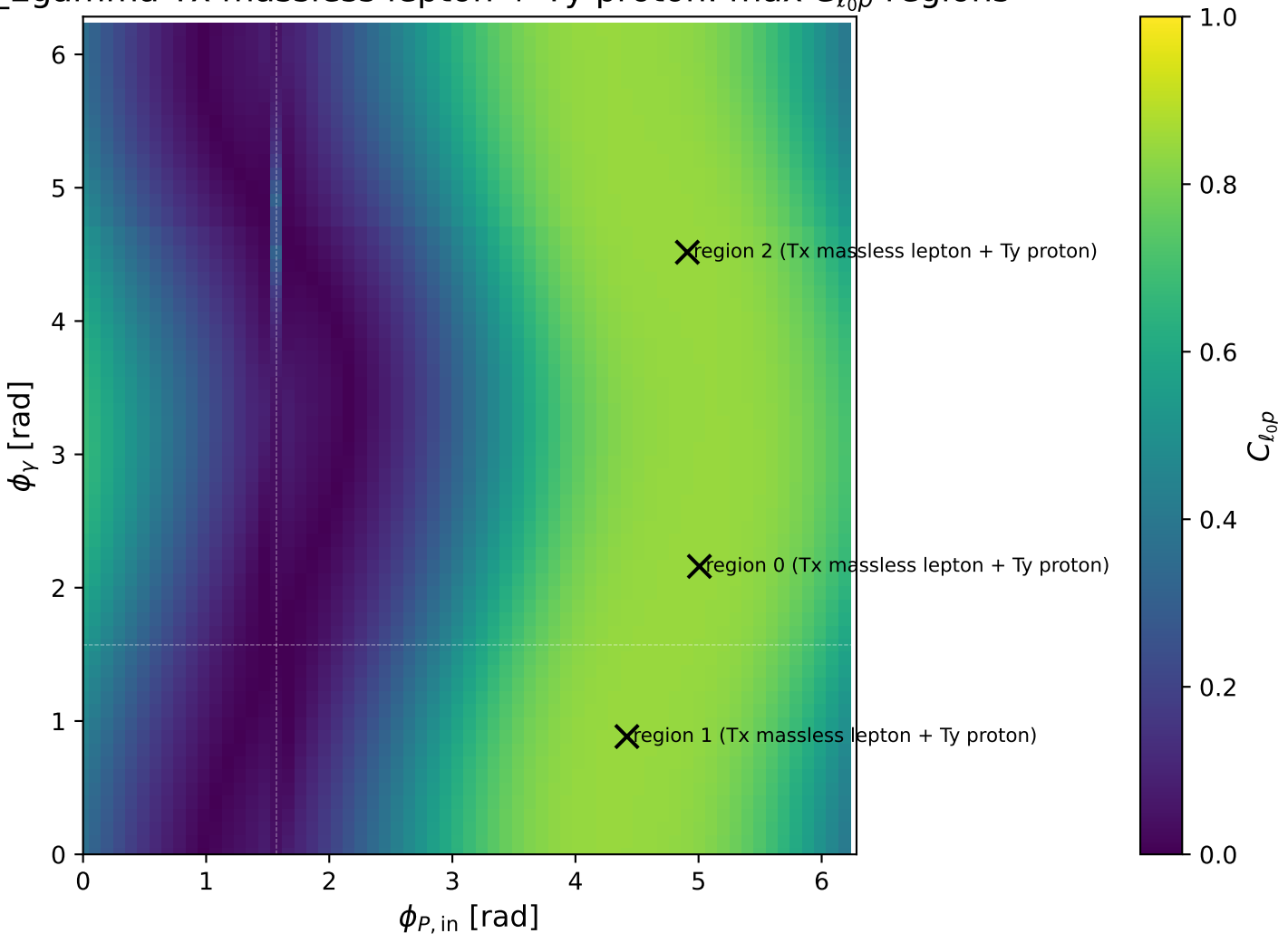
Gamma Tx massless lepton + Ty proton: max C_{\ell_0 p} regions
