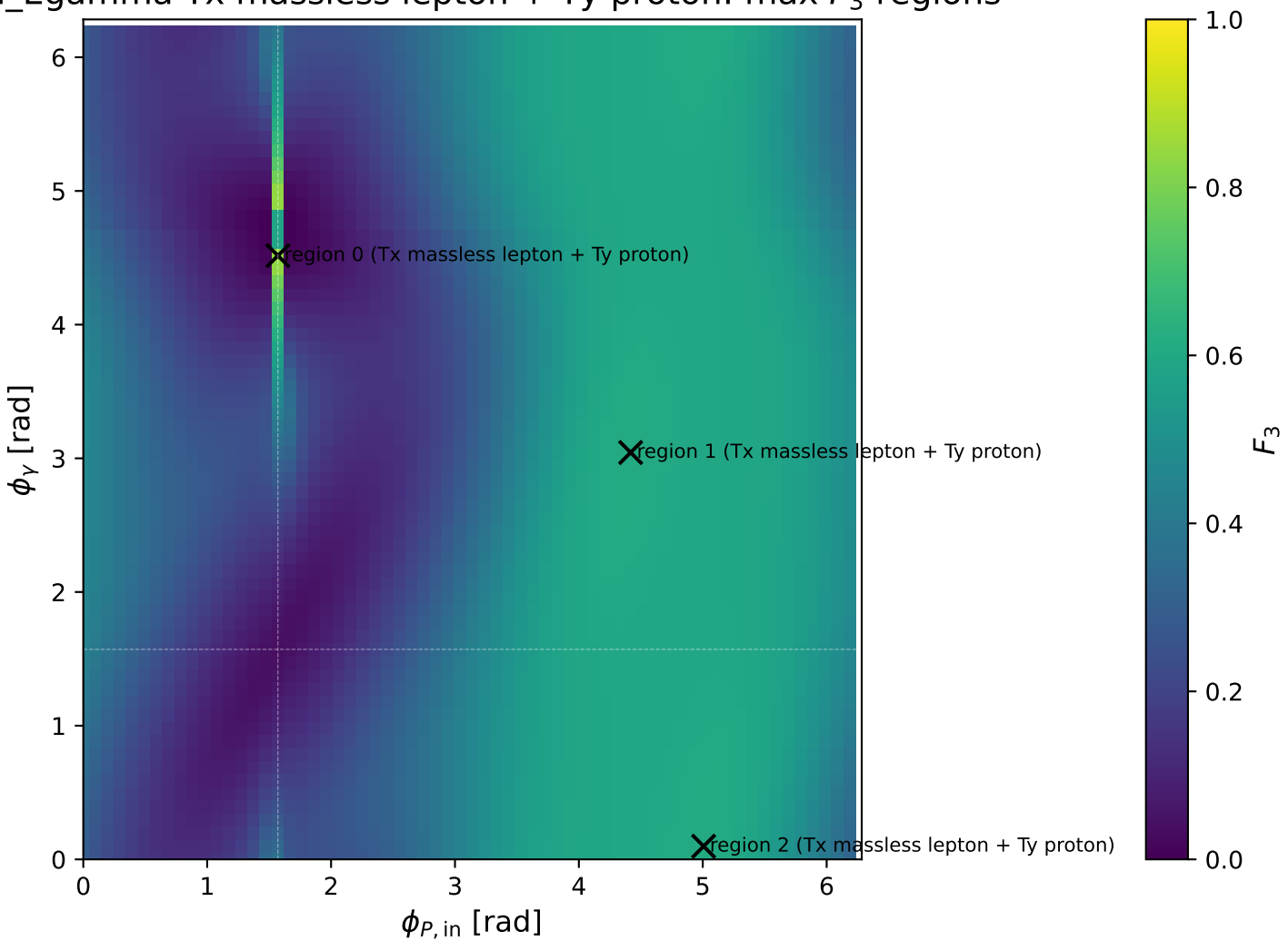
_Egamma Tx massless lepton + Ty proton: max F_3 regions
