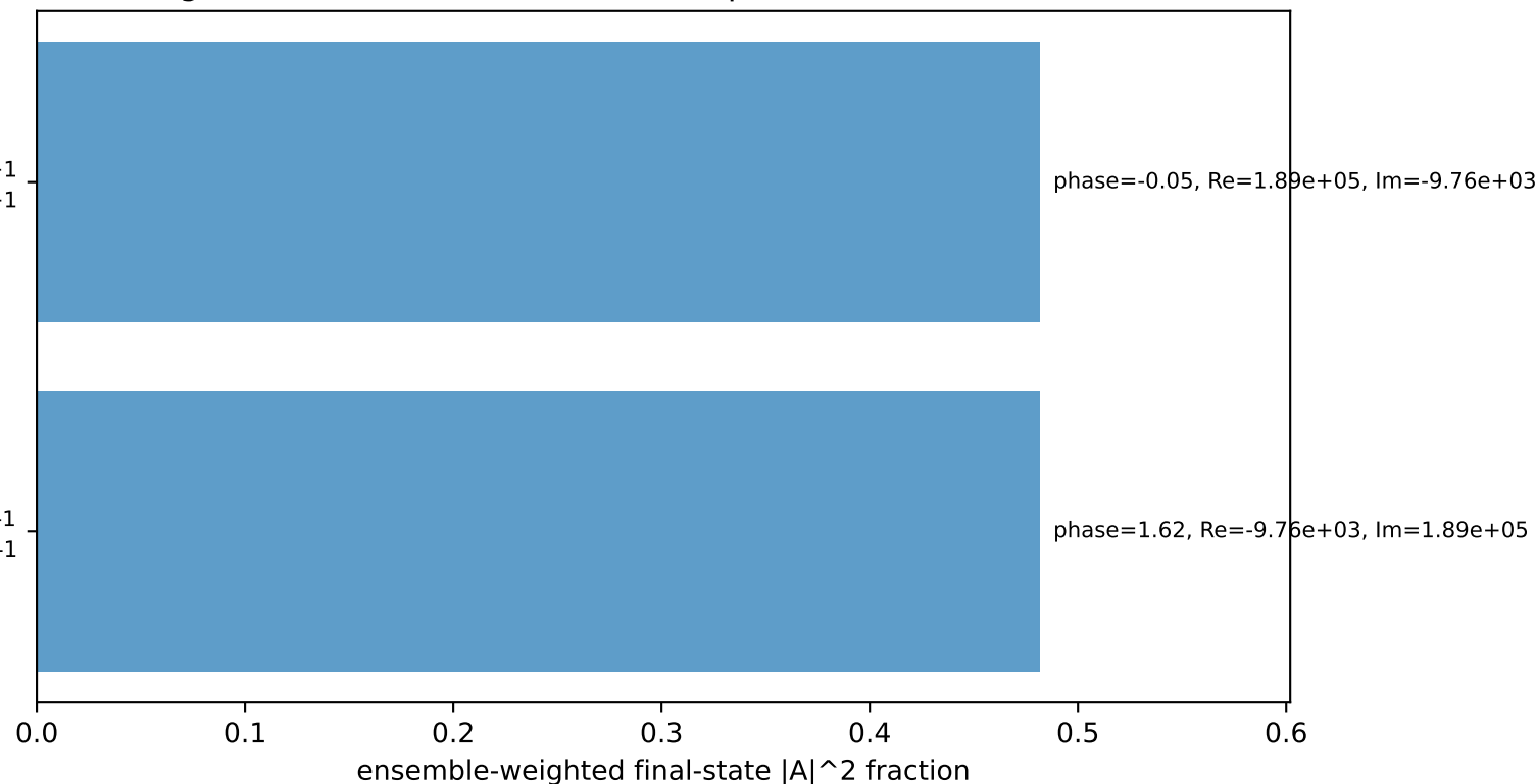
Leading initial-ensemble/final-state components (N=2, retained=96.3%)
