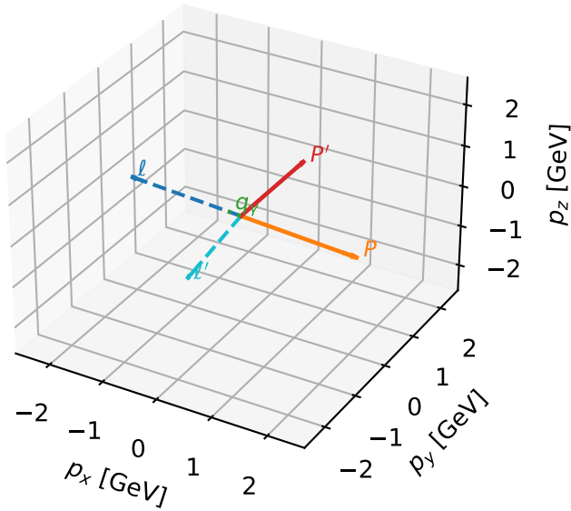
3D momenta
