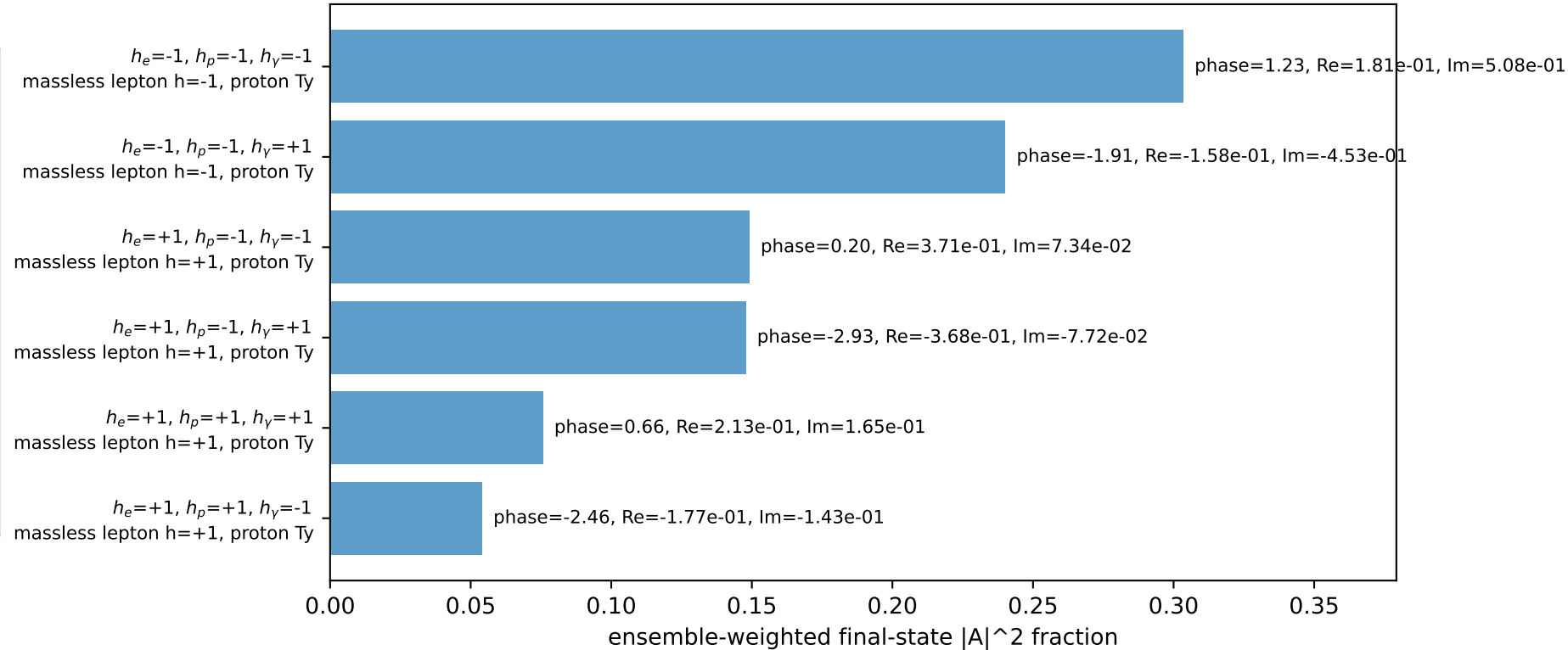
Leading initial-ensemble/final-state components (N=6, retained=97.0%)
