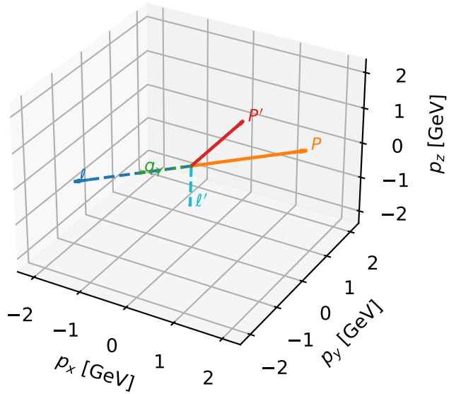
3D momenta
