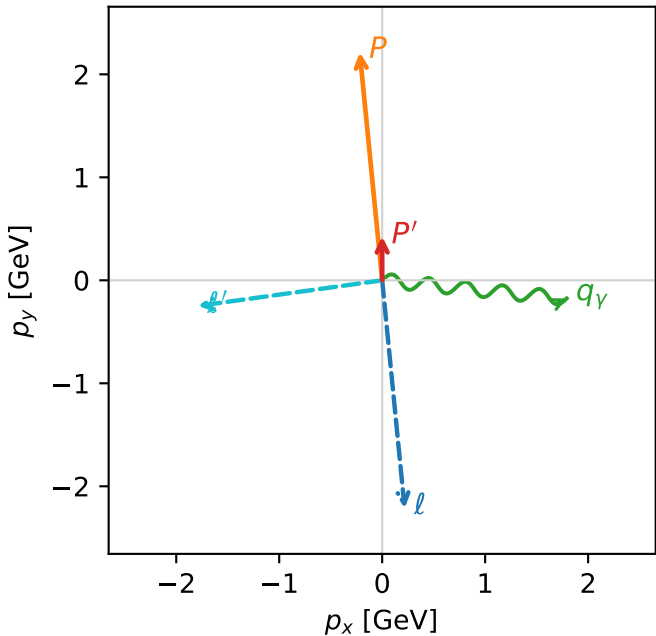
Transverse plane
