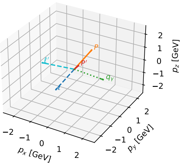
3D momenta
