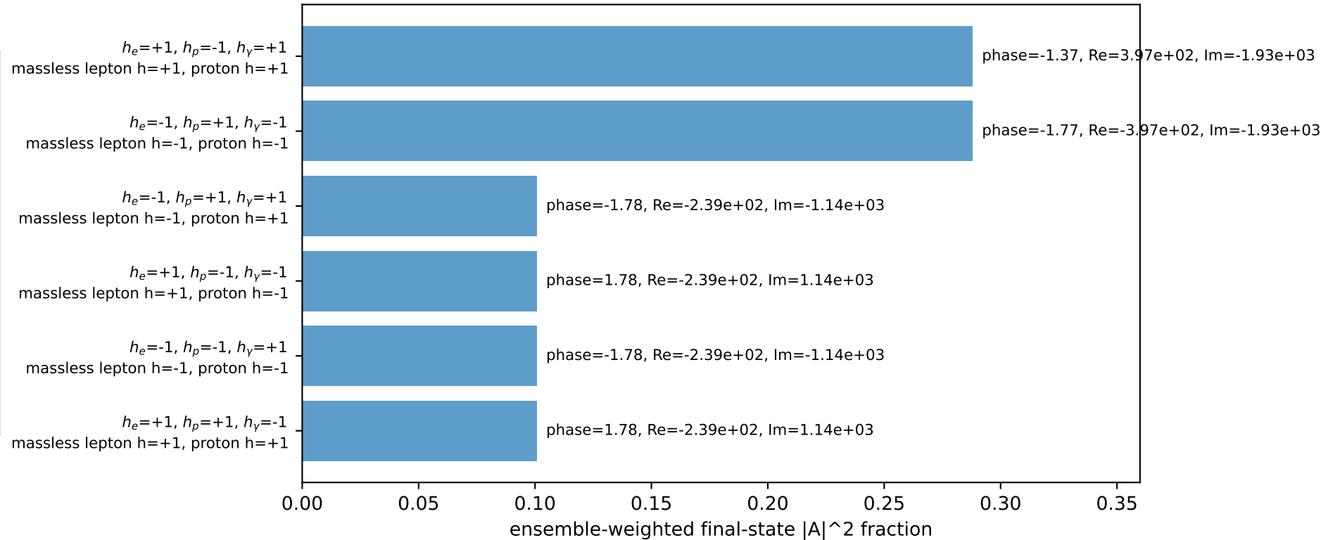
Leading initial-ensemble/final-state components (N=6, retained=97.9%)
