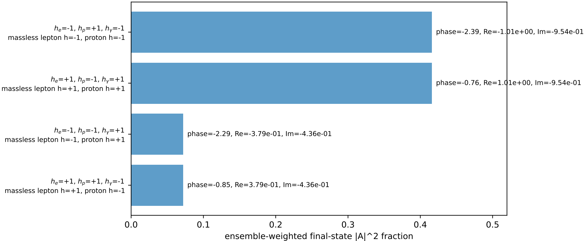
Leading initial-ensemble/final-state components (N=4, retained=97.6%)
