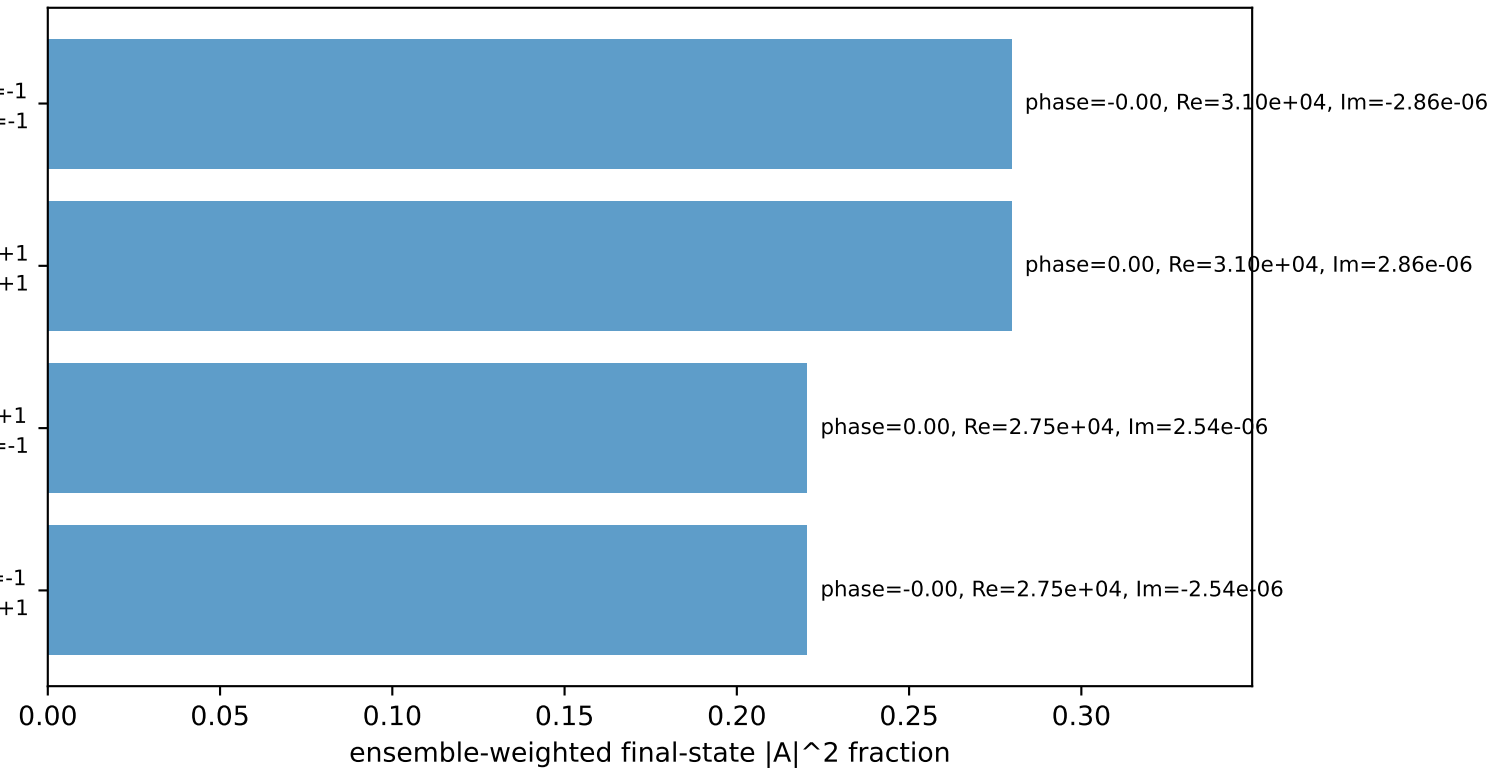
Leading initial-ensemble/final-state components (N=4, retained=100.0%)
