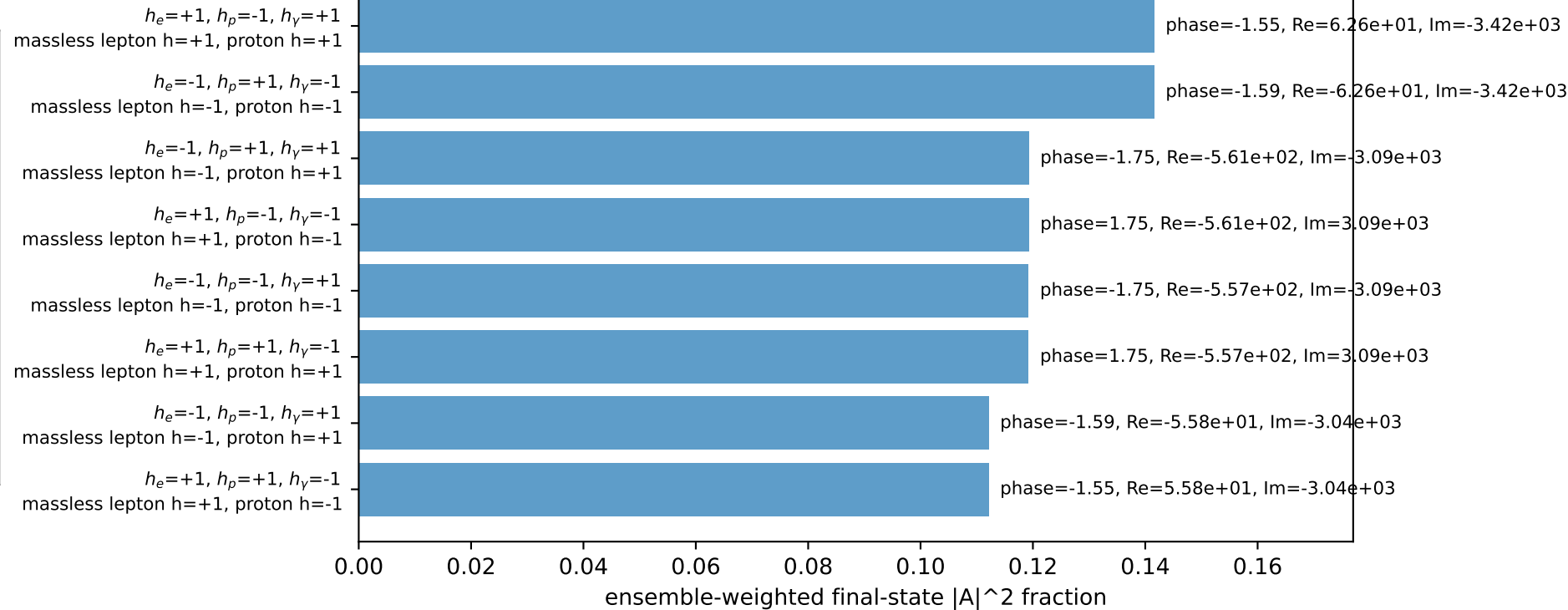
Leading initial-ensemble/final-state components (N=8, retained=98.5%)
