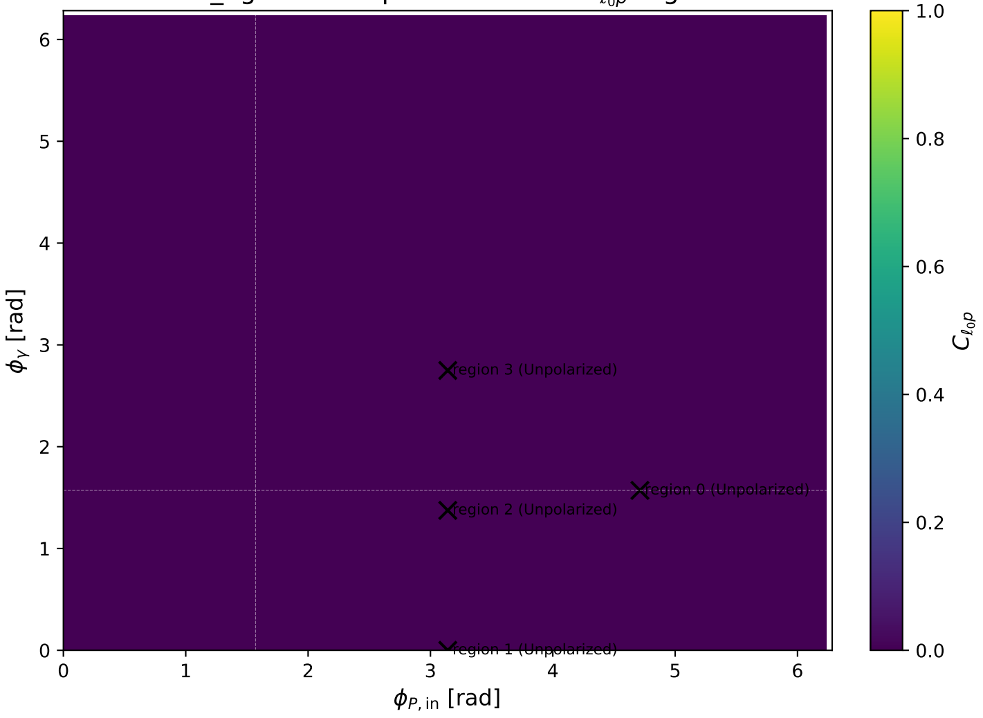
mid_Egamma Unpolarized: max C_{\ell_0 p} regions
