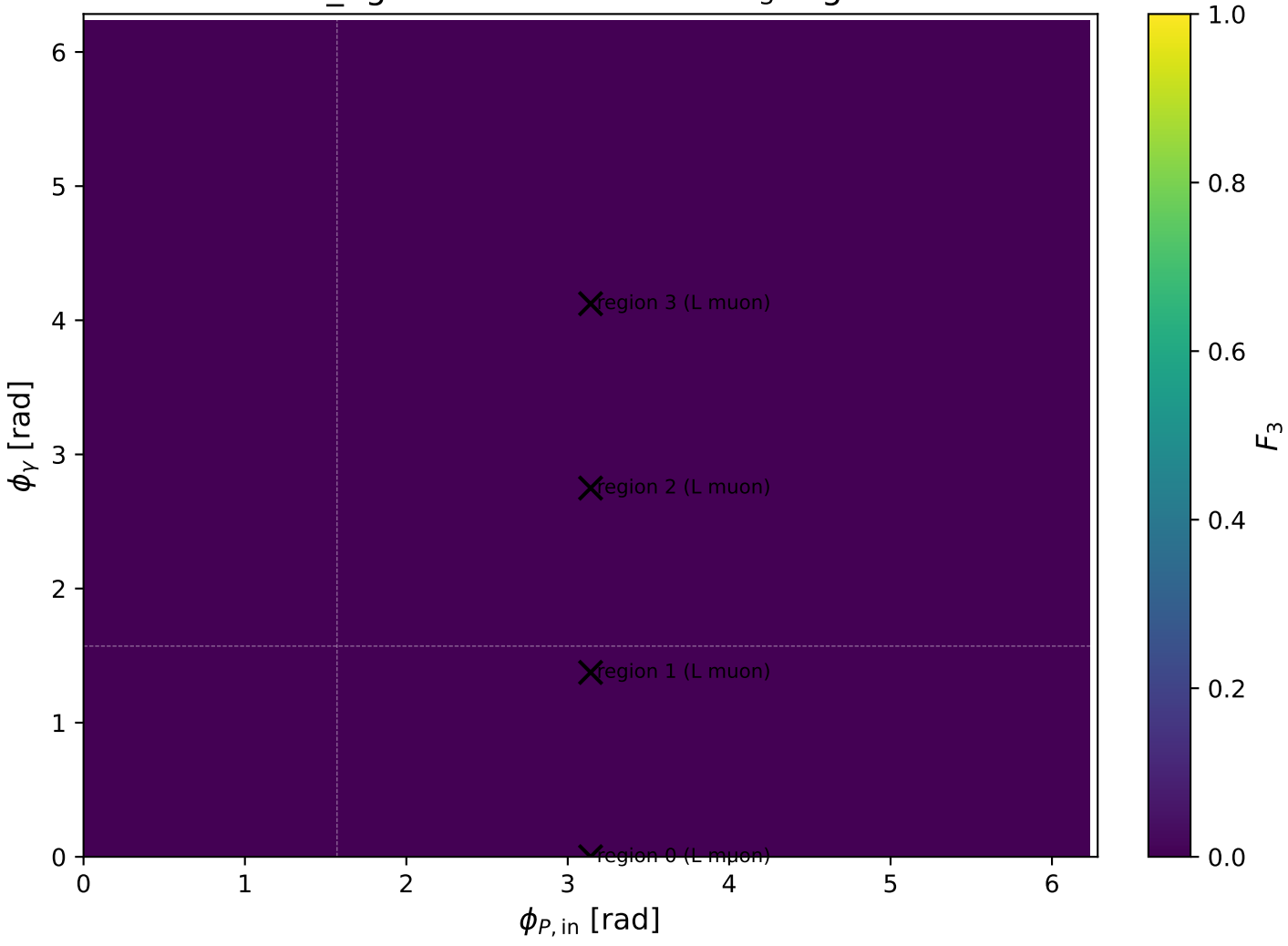
low_Egamma L muon: max F_3 regions
