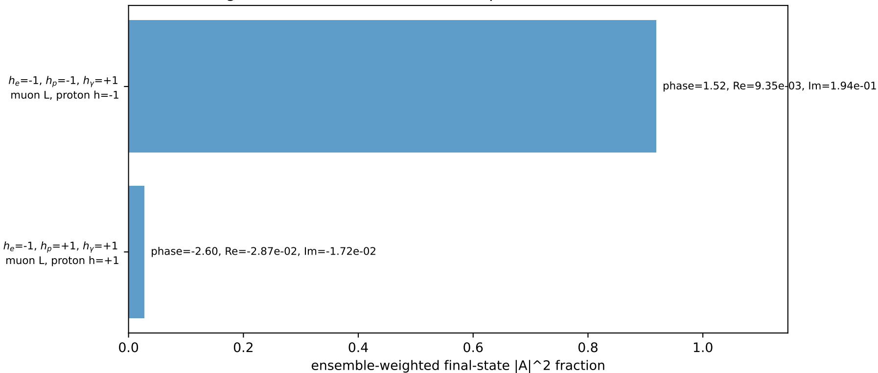
Leading initial-ensemble/final-state components (N=2, retained=94.6%)
