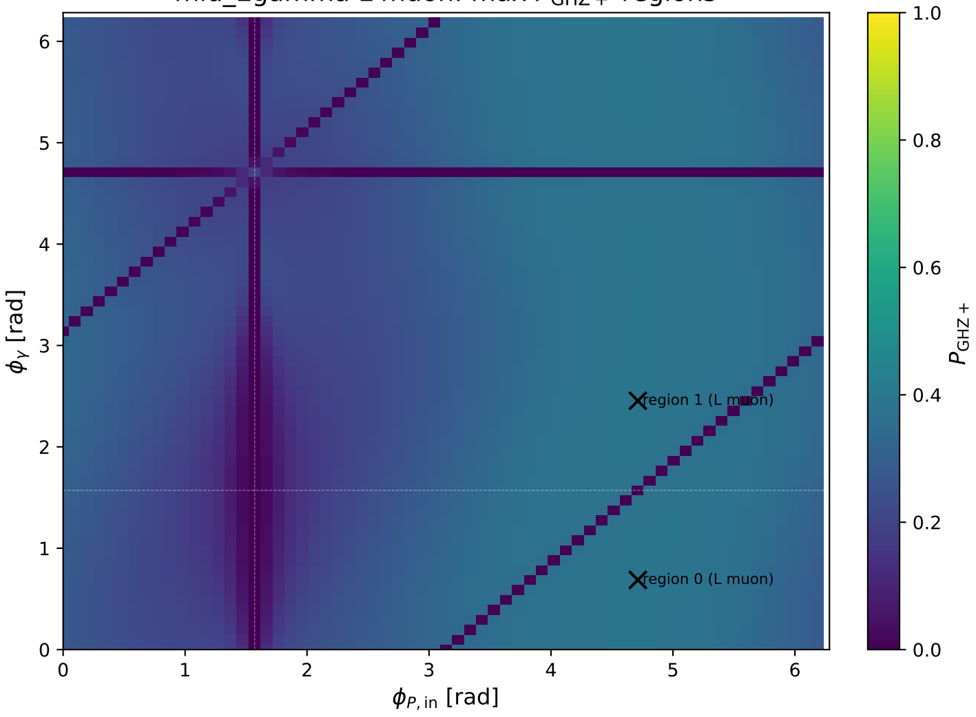
mid_Egamma L muon: max P_{\text{GHZ}+} regions
