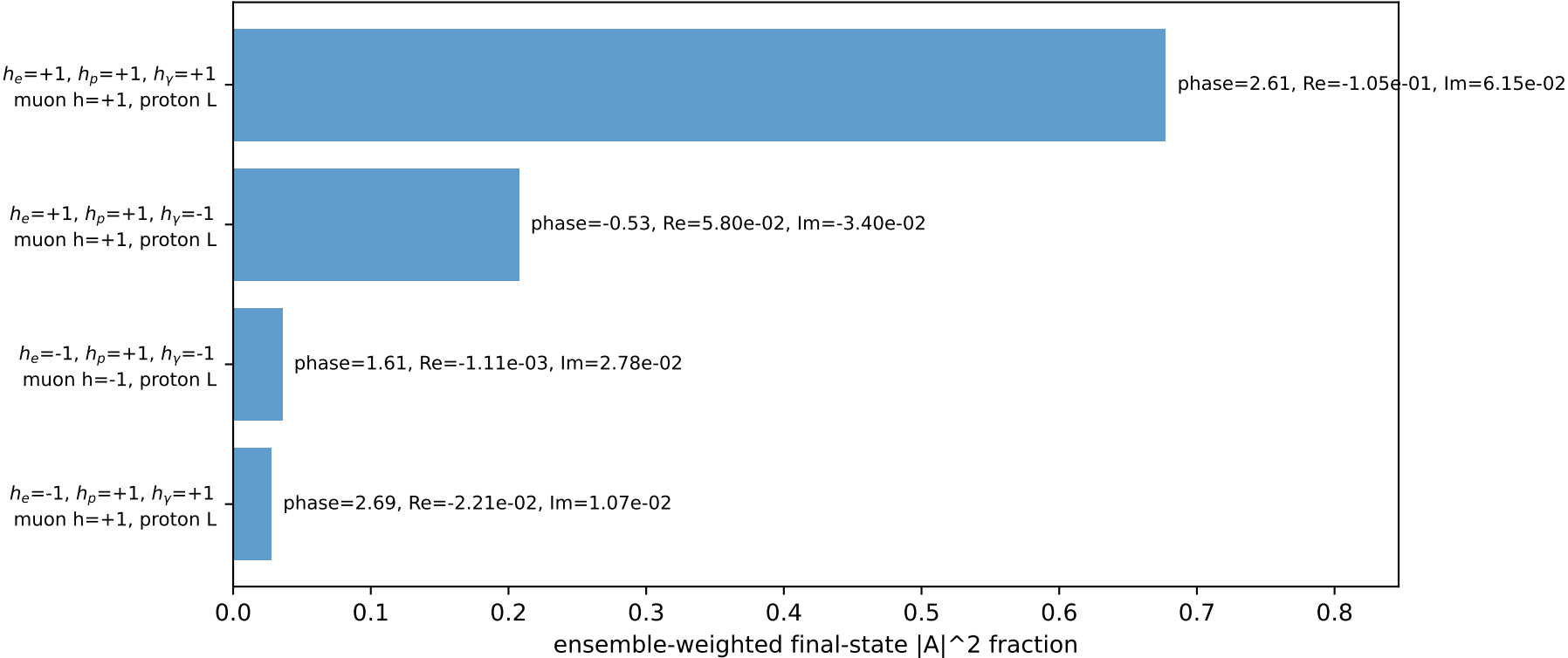
Leading initial-ensemble/final-state components (N=4, retained=94.8%)
