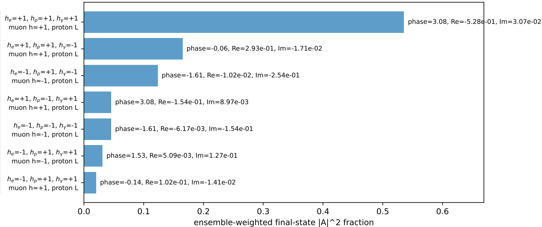
Leading initial-ensemble/final-state components (N=7, retained=96.6%)
