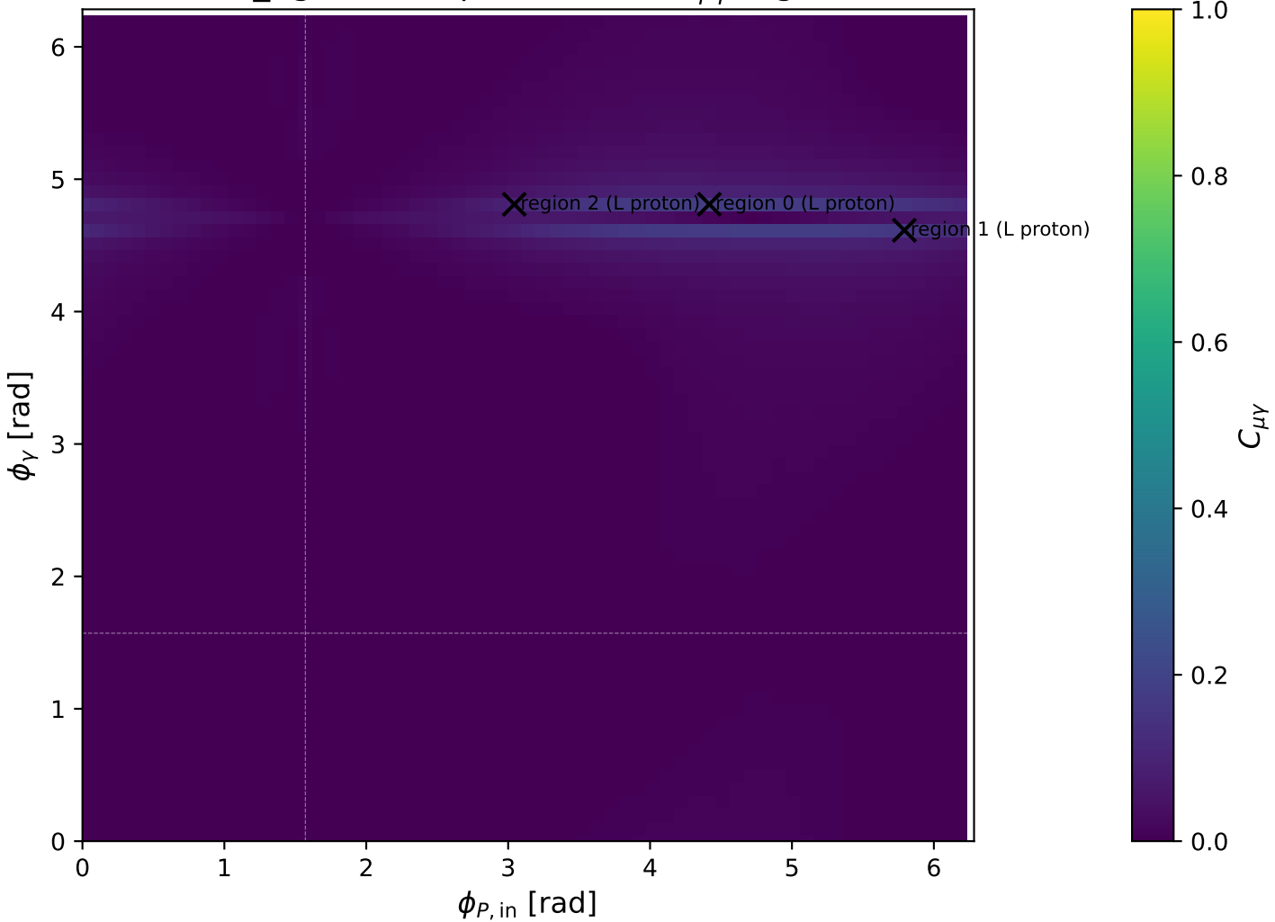
mid_Egamma L proton: max C_{\mu\gamma} regions
