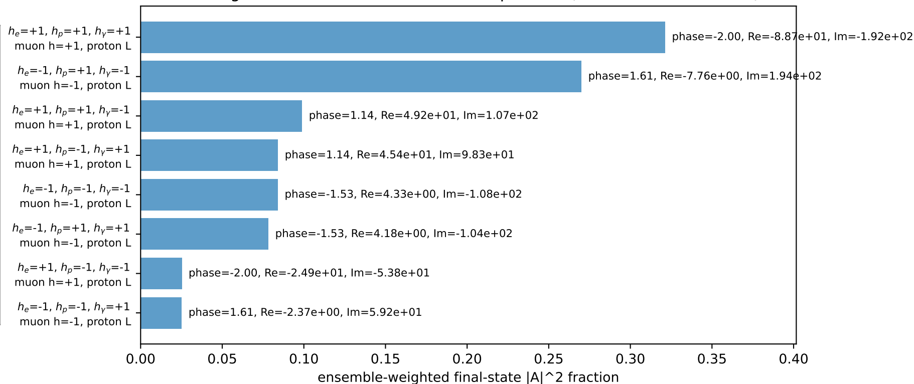
Leading initial-ensemble/final-state components (N=8, retained=98.7%)
