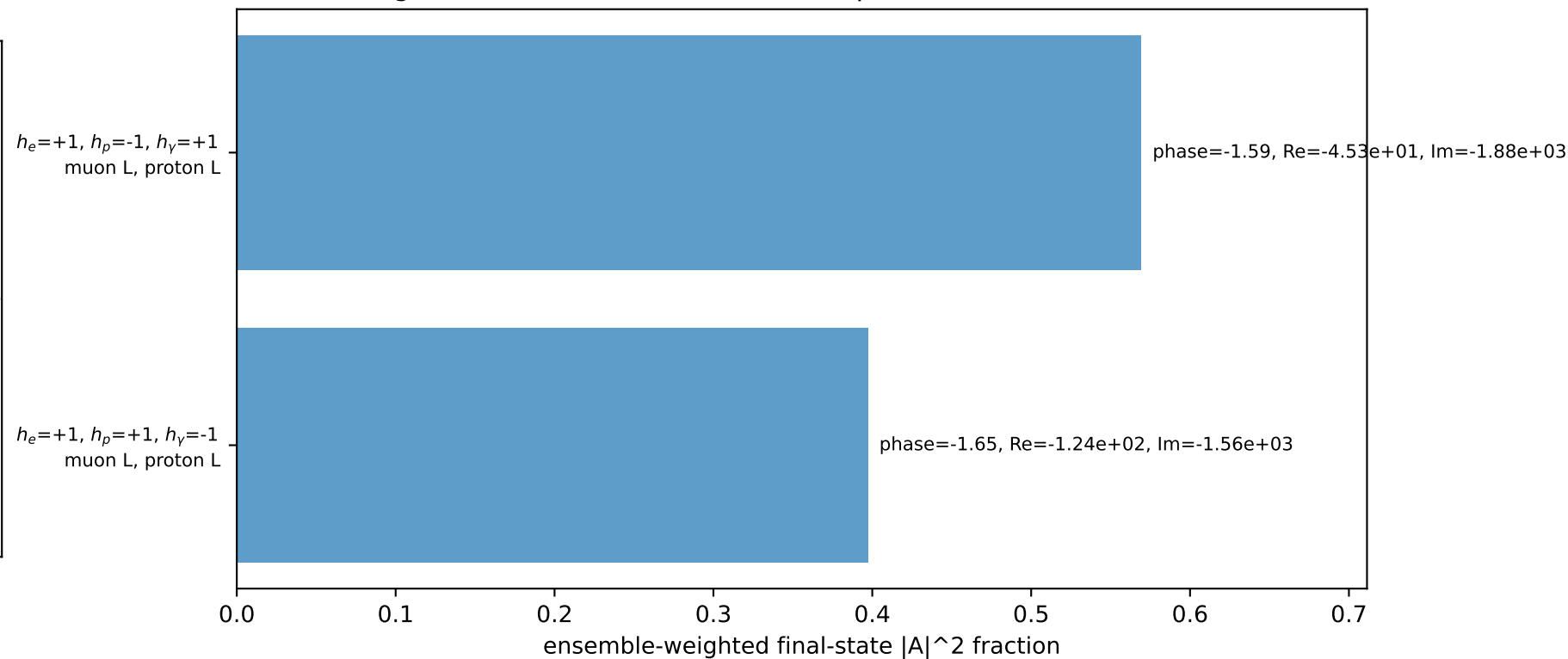
Leading initial-ensemble/final-state components (N=2, retained=96.6%)
