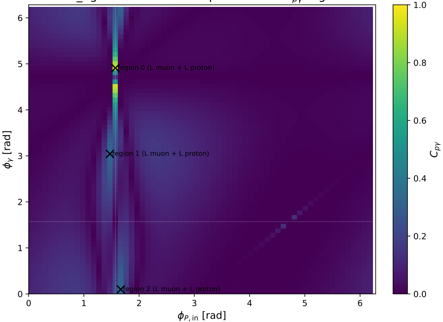
mid_Egamma L muon + L proton: max C_{p\gamma} regions
