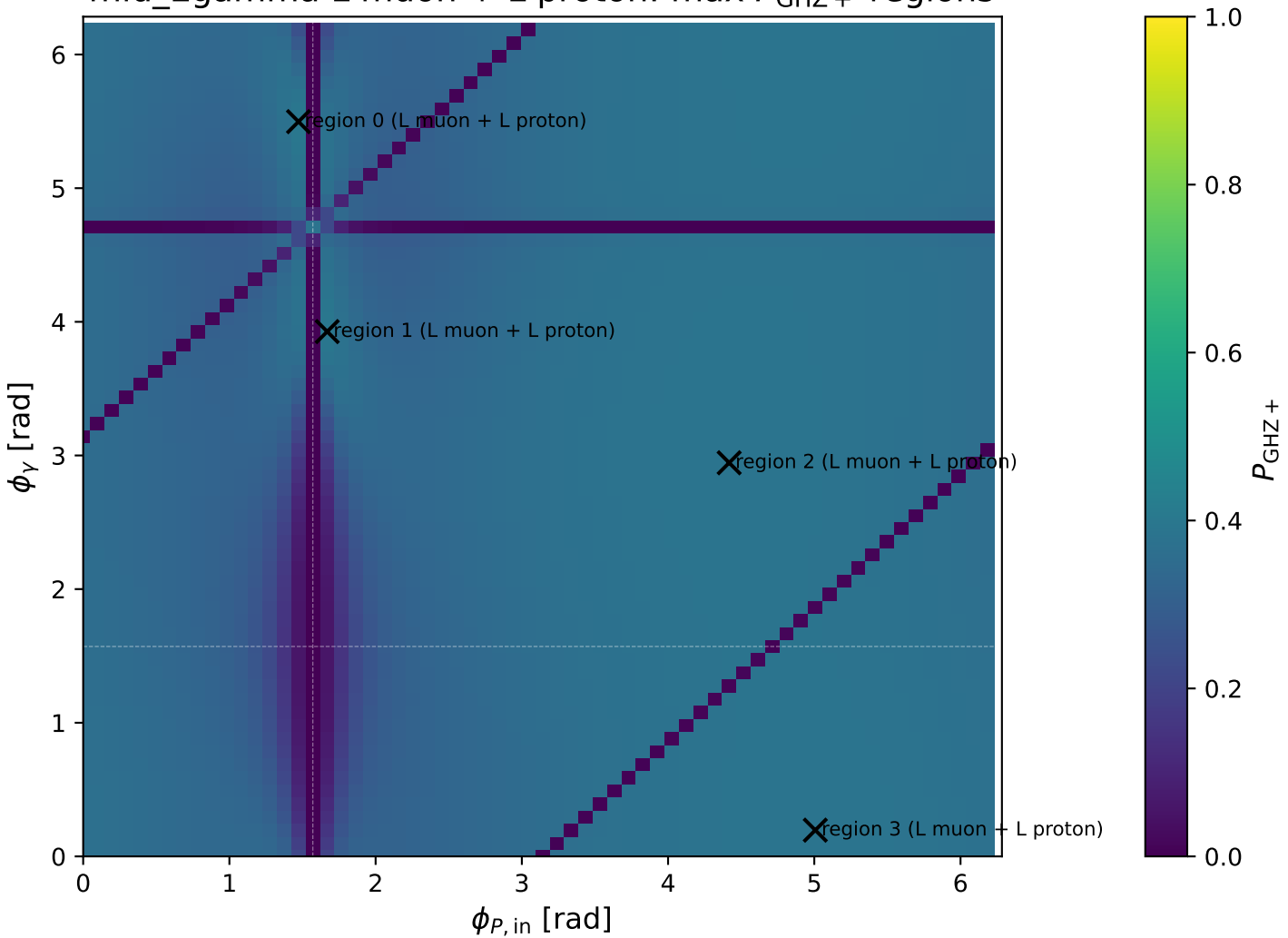
mid_Egamma L muon + L proton: max P_{\text{GHZ}} + regions
