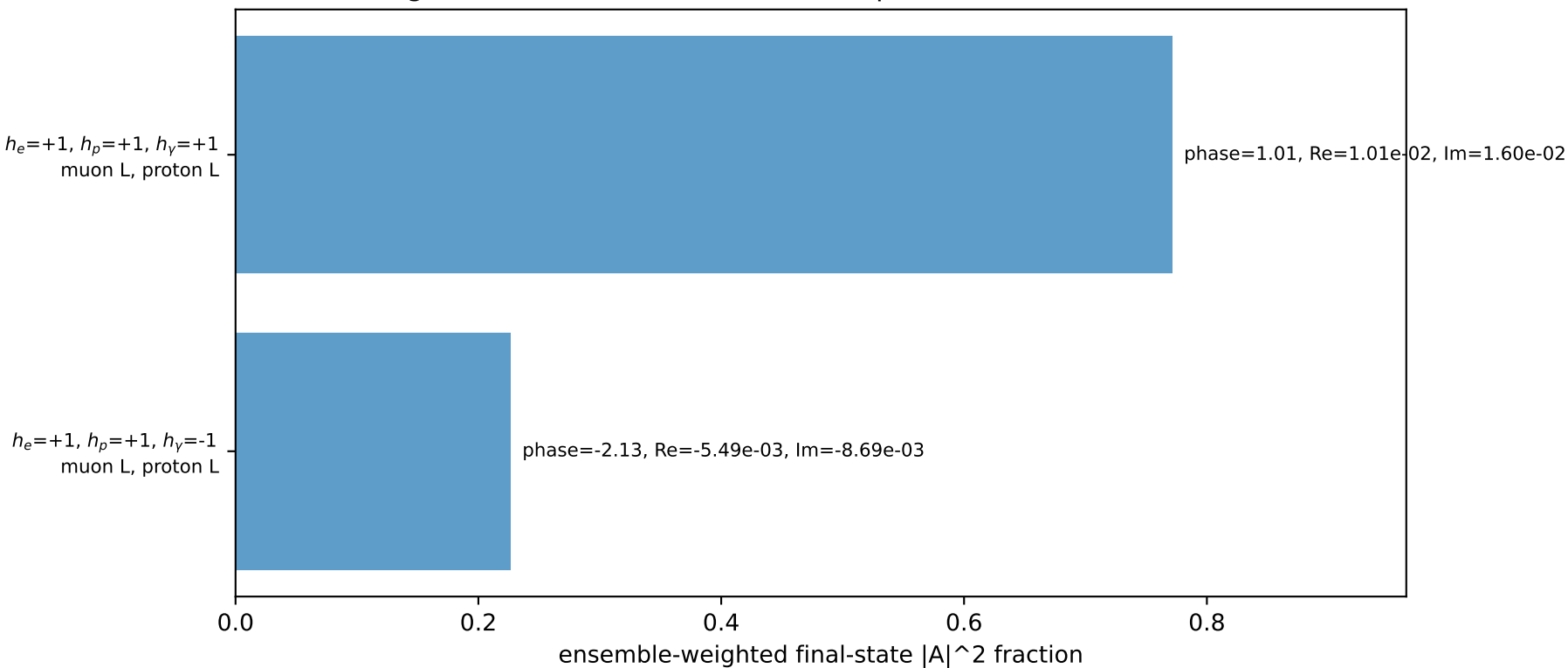
Leading initial-ensemble/final-state components (N=2, retained=99.8%)
