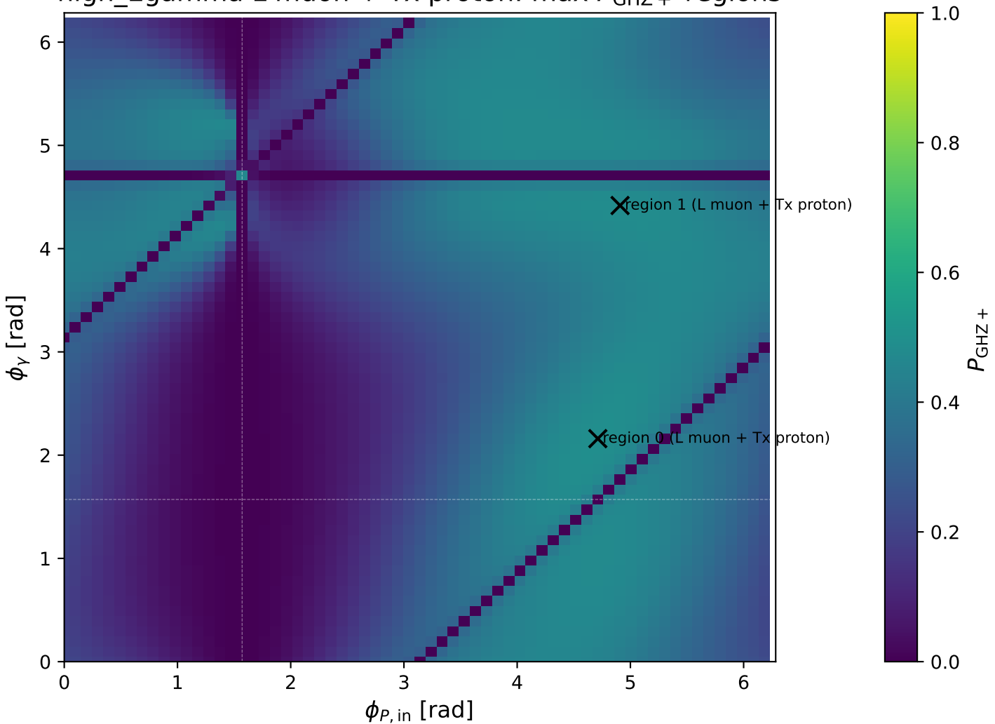
high_Egamma L muon + Tx proton: max P_{\text{GHZ}} + regions
