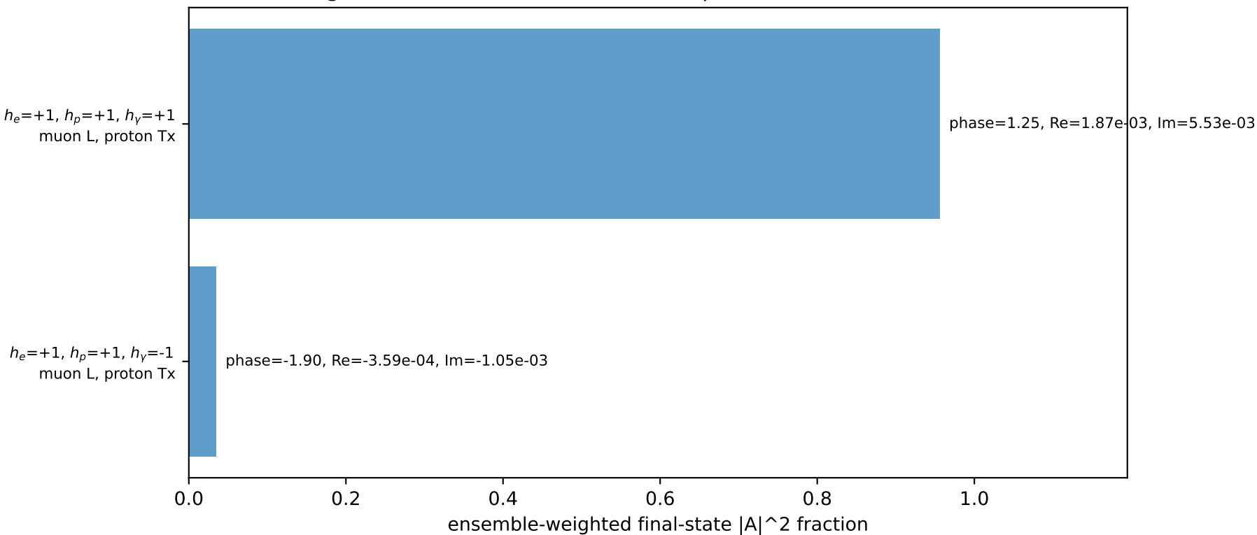
Leading initial-ensemble/final-state components (N=2, retained=99.1%)
