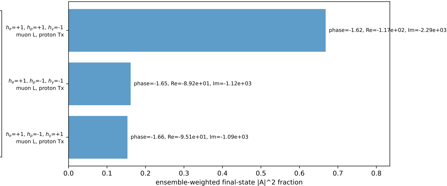
Leading initial-ensemble/final-state components (N=3, retained=98.2%)
