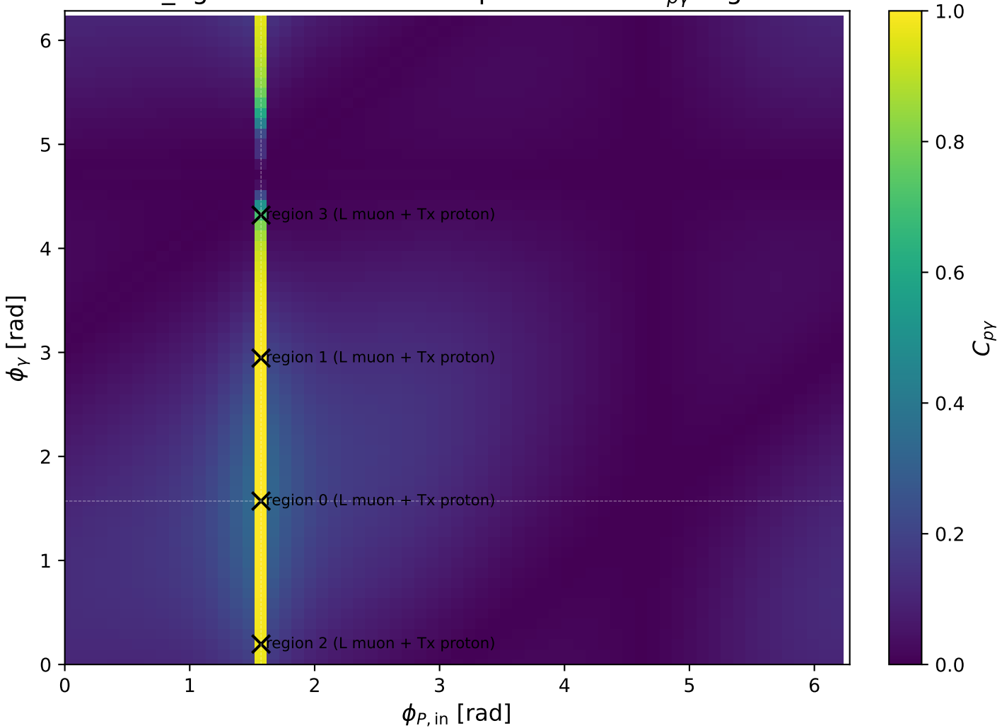
low_Egamma L muon + Tx proton: max C_{p\gamma} regions
