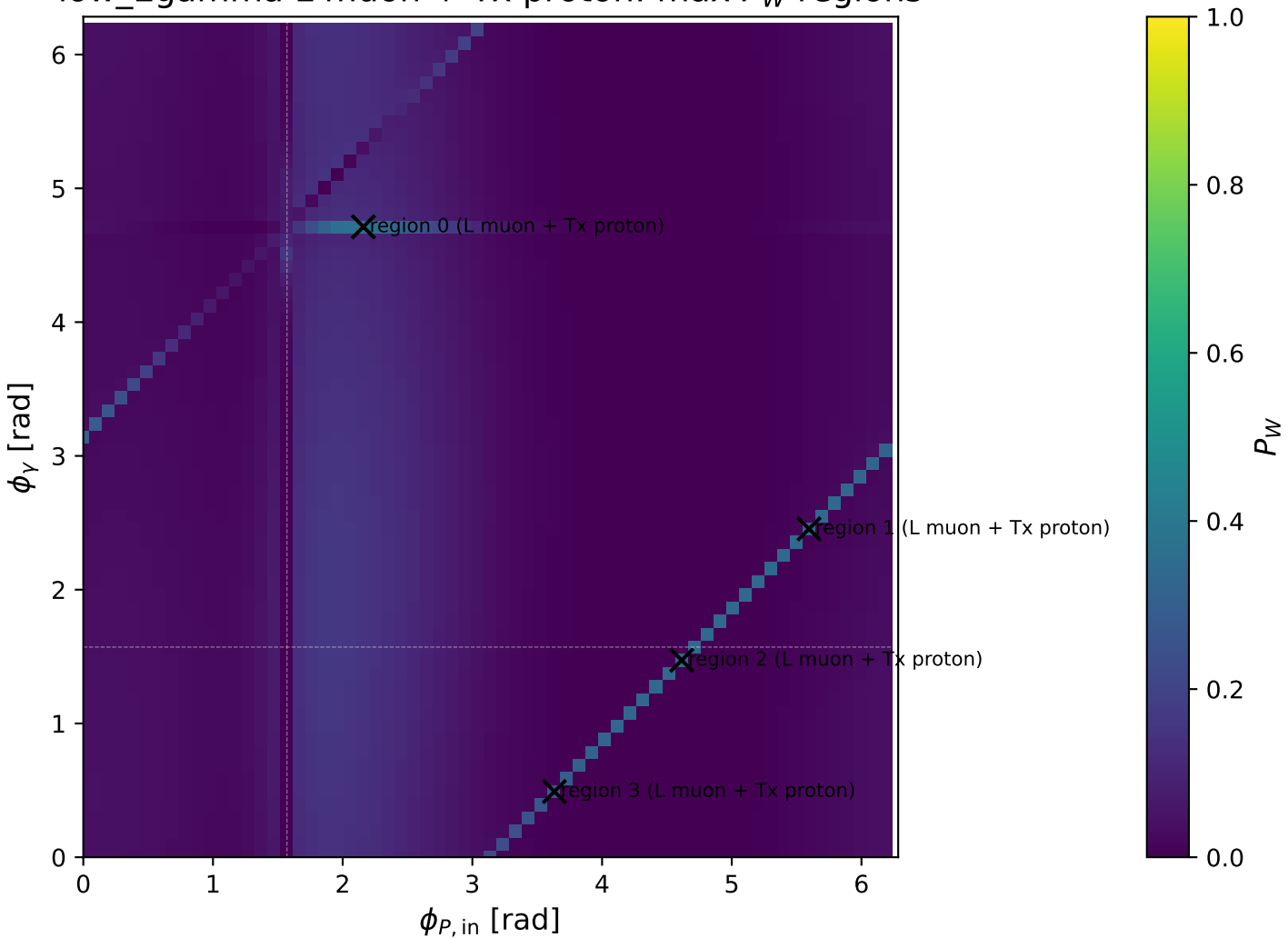
low_Egamma L muon + Tx proton: max P_W regions
