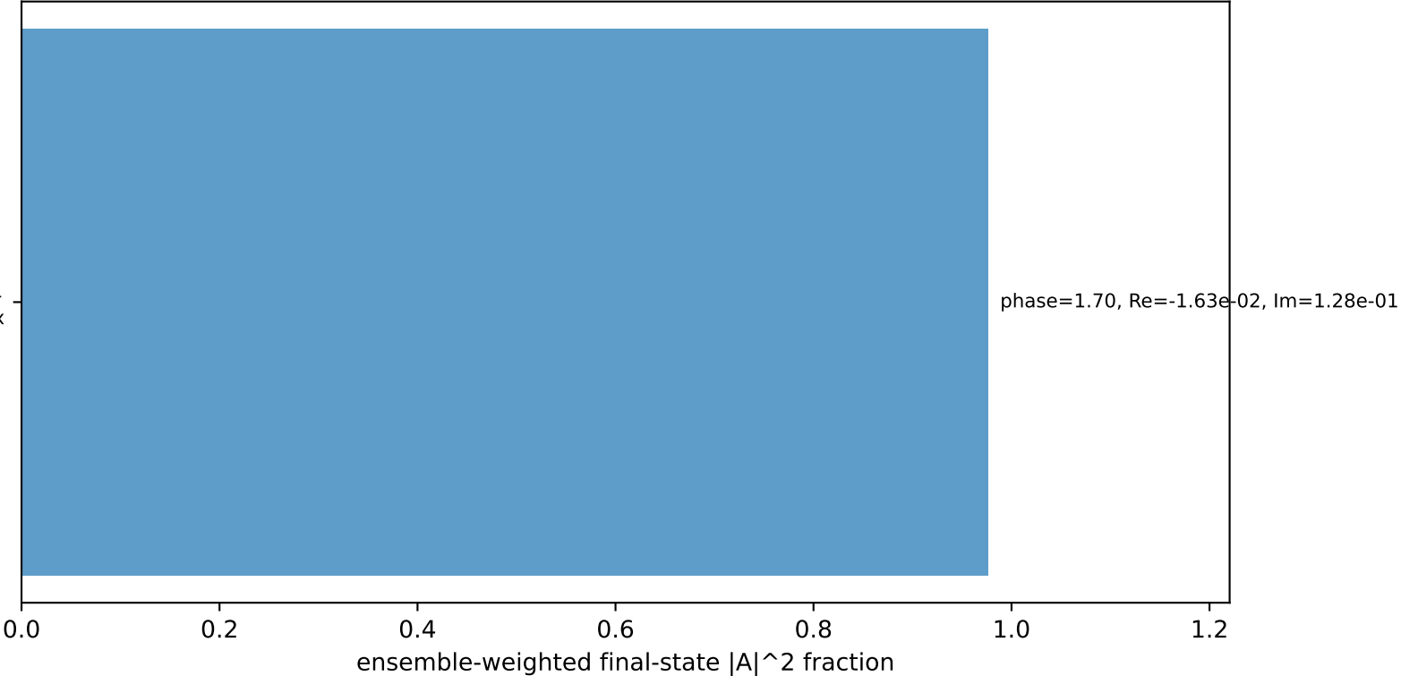
Leading initial-ensemble/final-state components (N=1, retained=97.6%)
