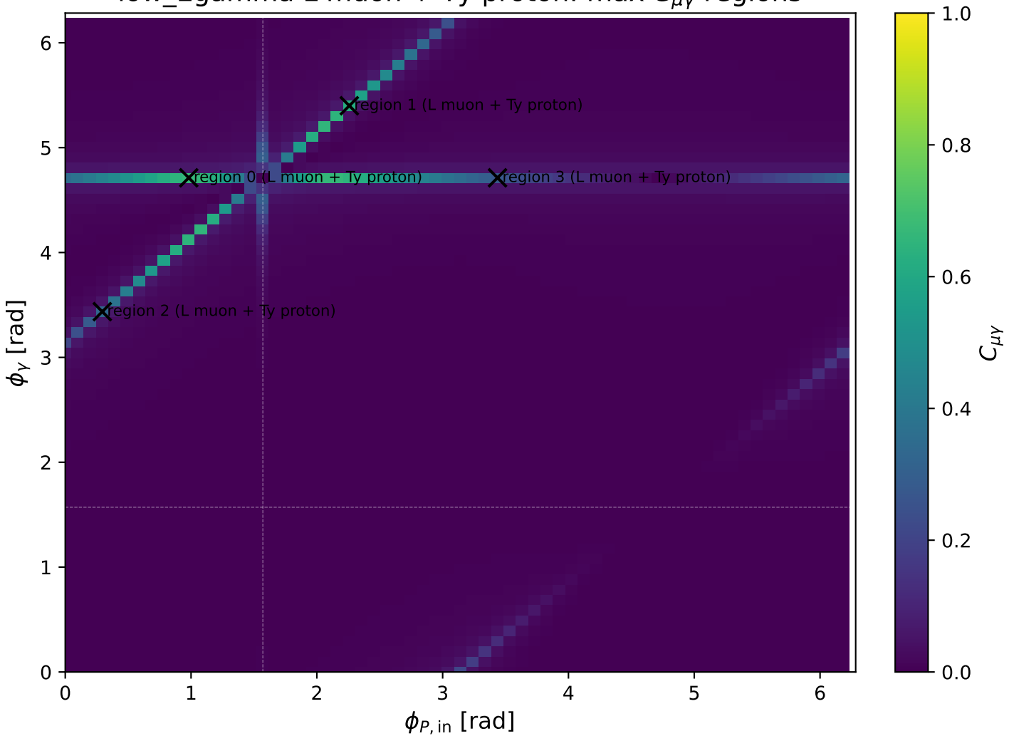
low_Egamma L muon + Ty proton: max C_{\mu\gamma} regions
