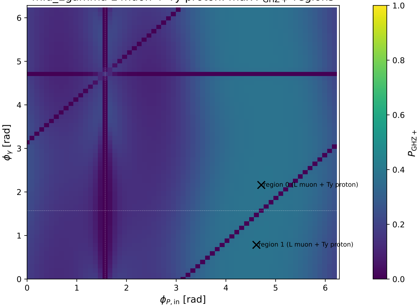
mid_Egamma L muon + Ty proton: max P_{\text{GHZ}} + regions
