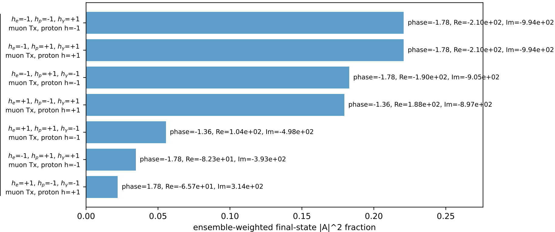
Leading initial-ensemble/final-state components (N=7, retained=91.5%)
