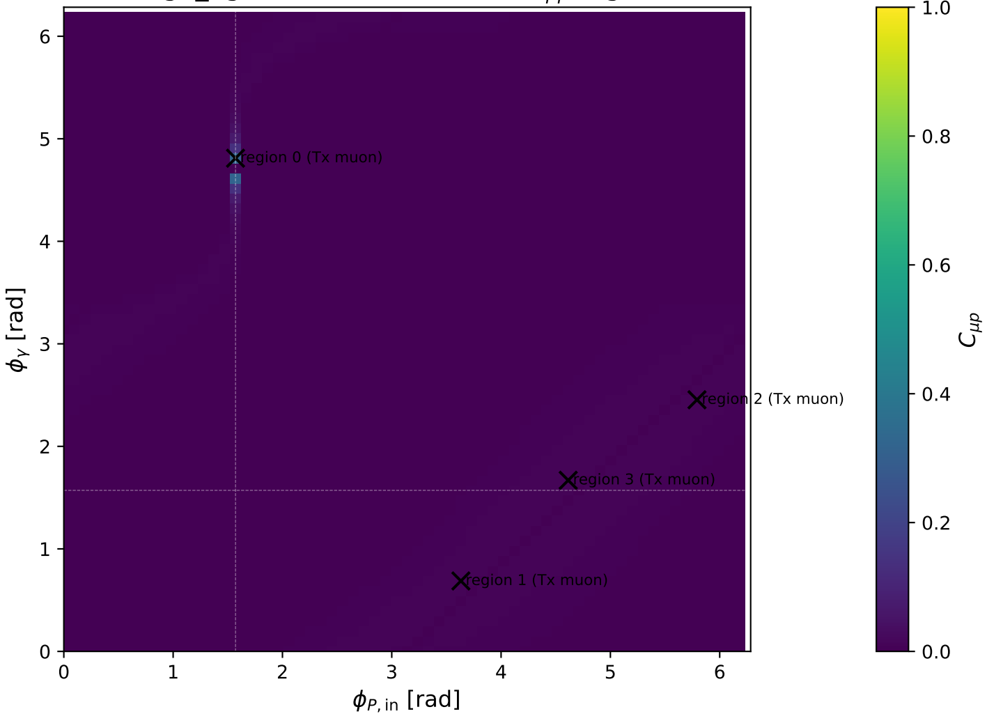
high_Egamma Tx muon: max C_{\mu p} regions
