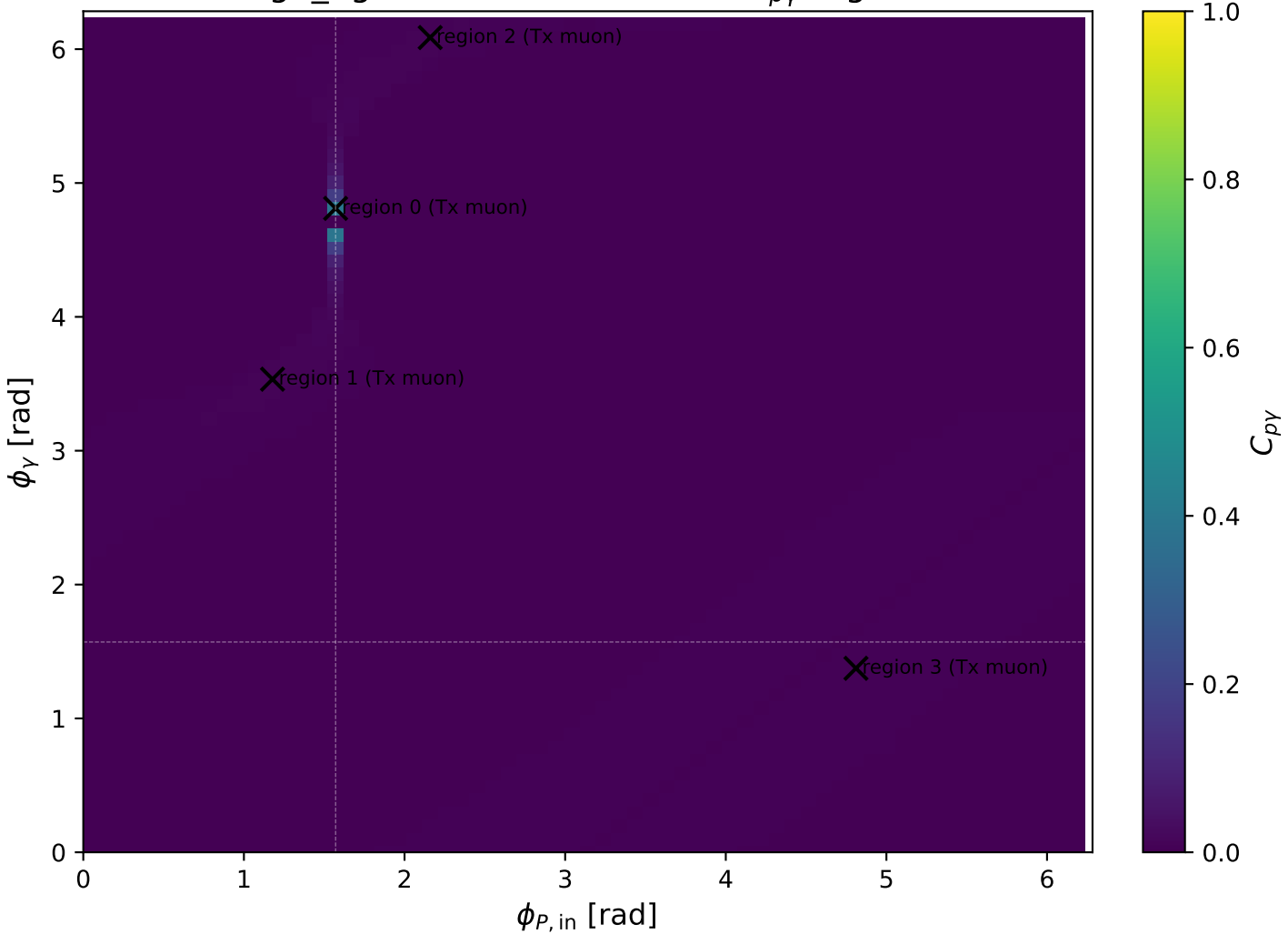
high_Egamma Tx muon: max C_{py} regions
