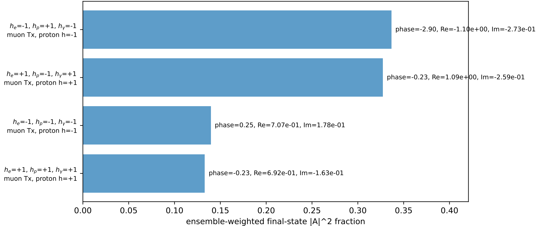
Leading initial-ensemble/final-state components (N=4, retained=93.6%)
