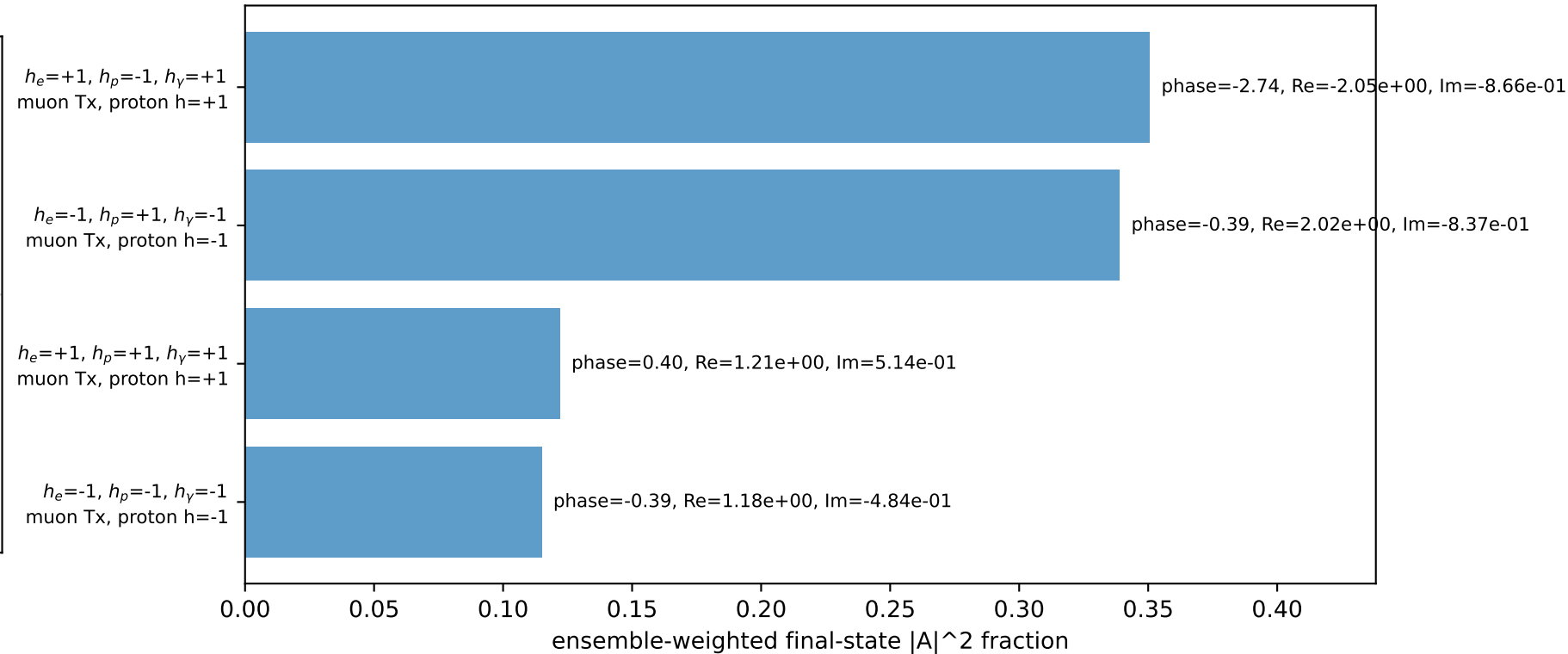
Leading initial-ensemble/final-state components (N=4, retained=92.6%)
