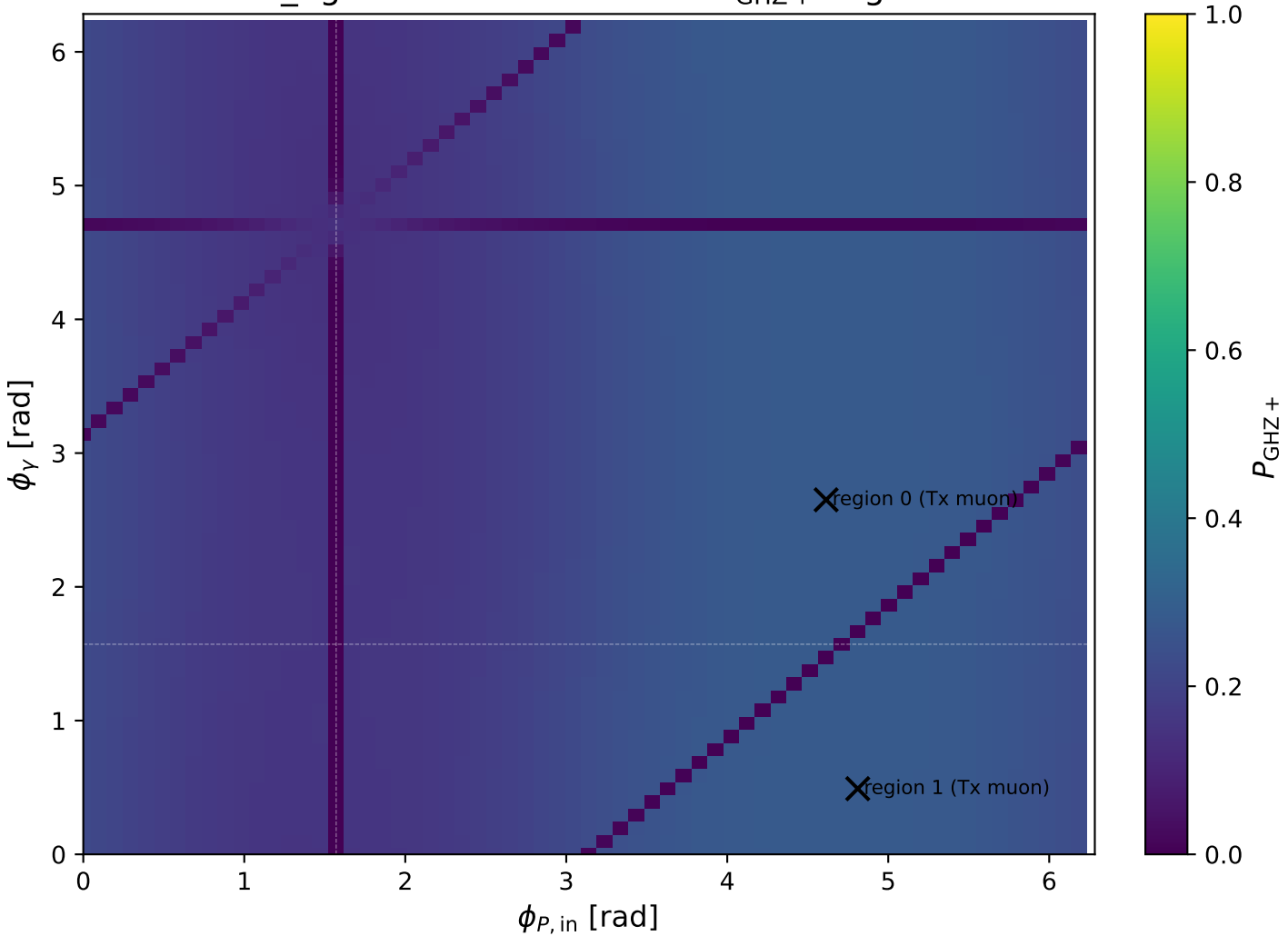
low_Egamma Tx muon: max P_{\text{GHz}+} regions
