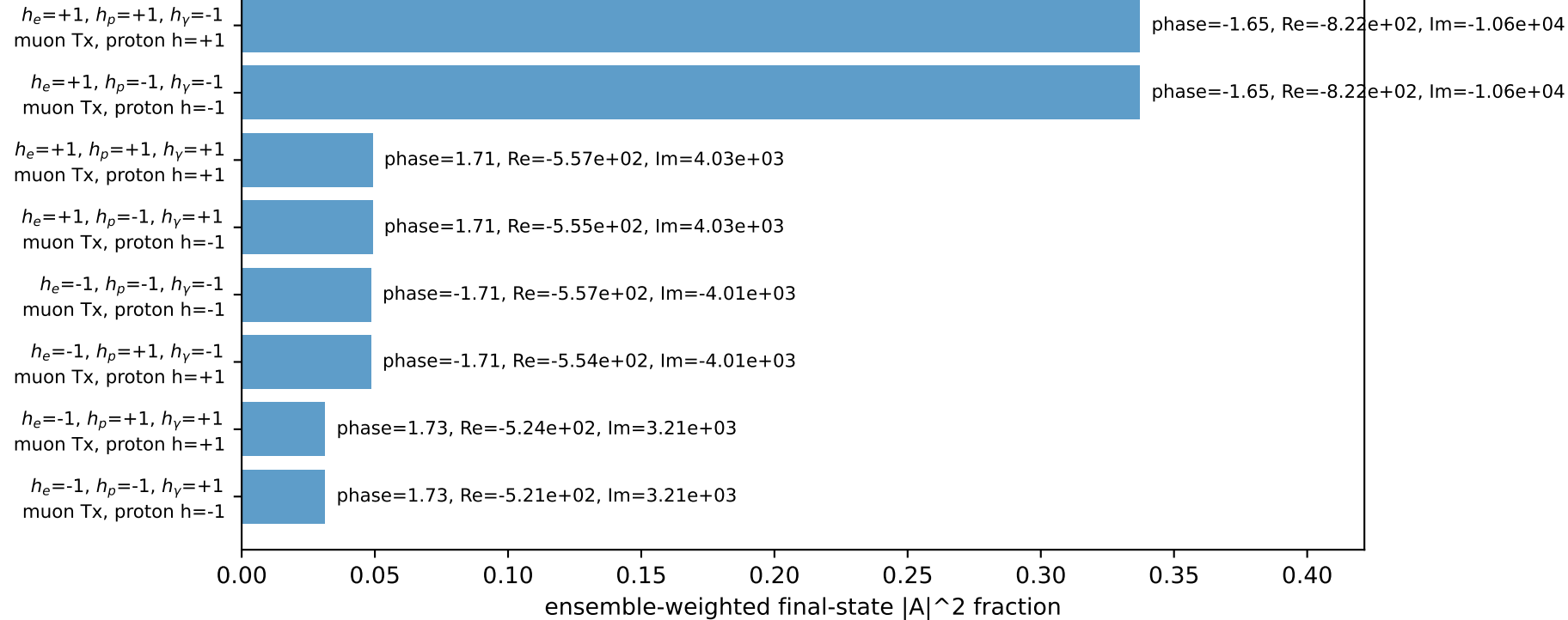
Leading initial-ensemble/final-state components (N=8, retained=93.2%)
