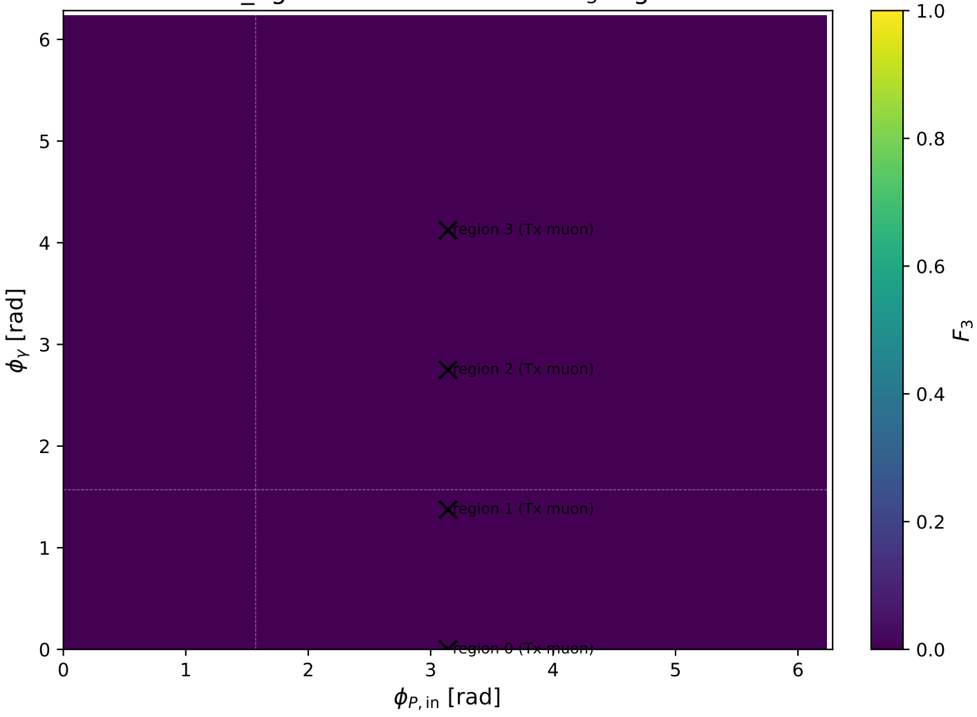
mid_Egamma Tx muon: max F_3 regions
