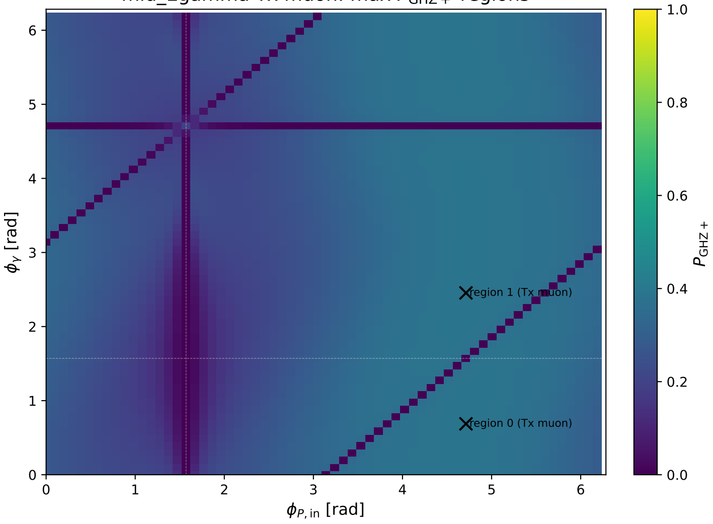
mid_Egamma Tx muon: max P_{\text{GHZ}+} regions
