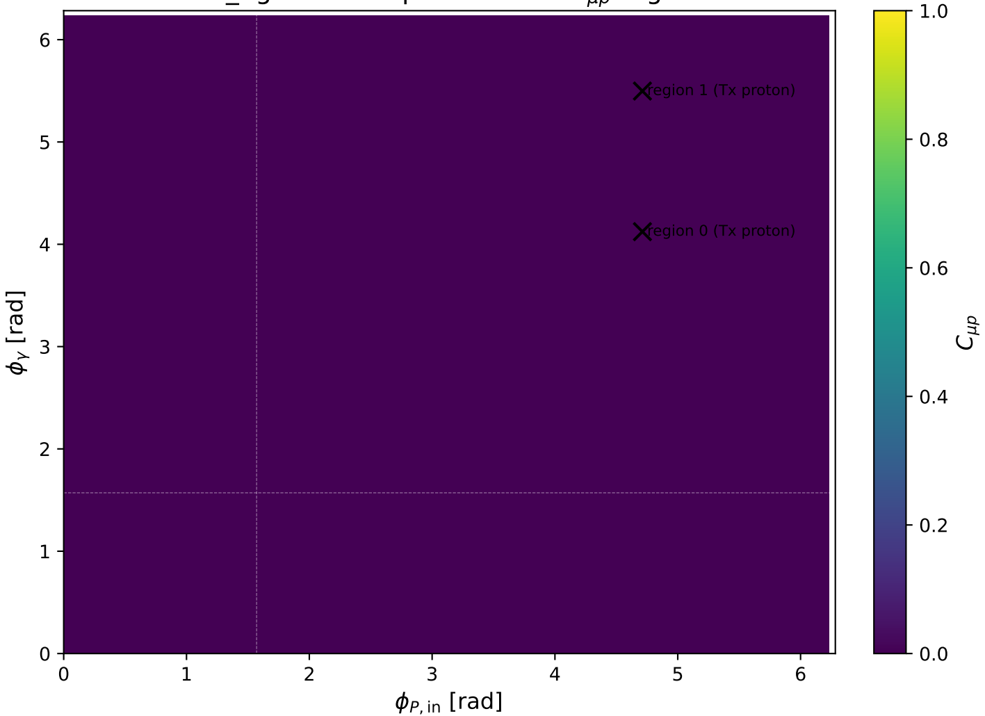
low_Egamma Tx proton: max C_{\mu p} regions
