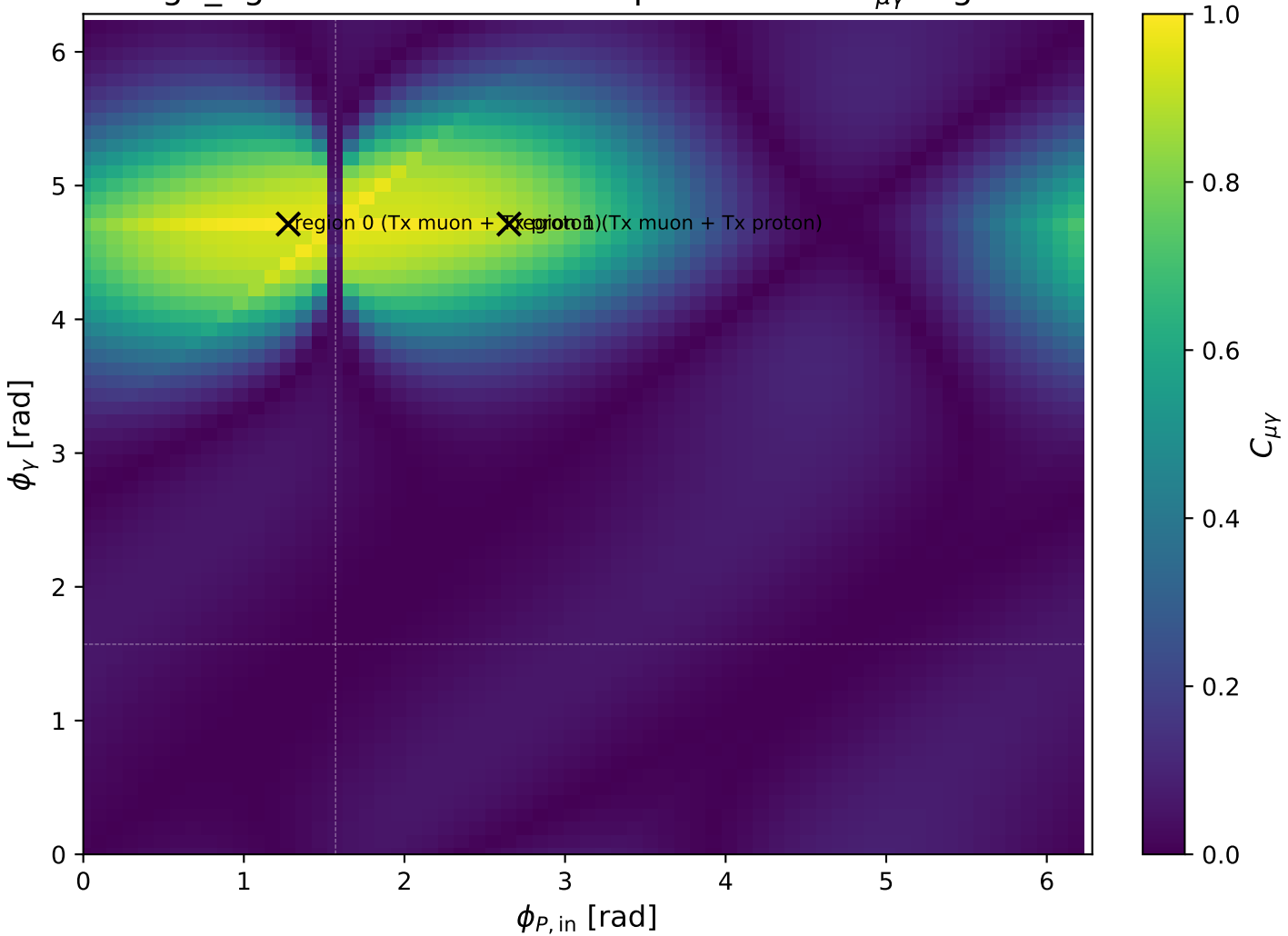
high_Egamma Tx muon + Tx proton: max C_{\mu\gamma} regions
