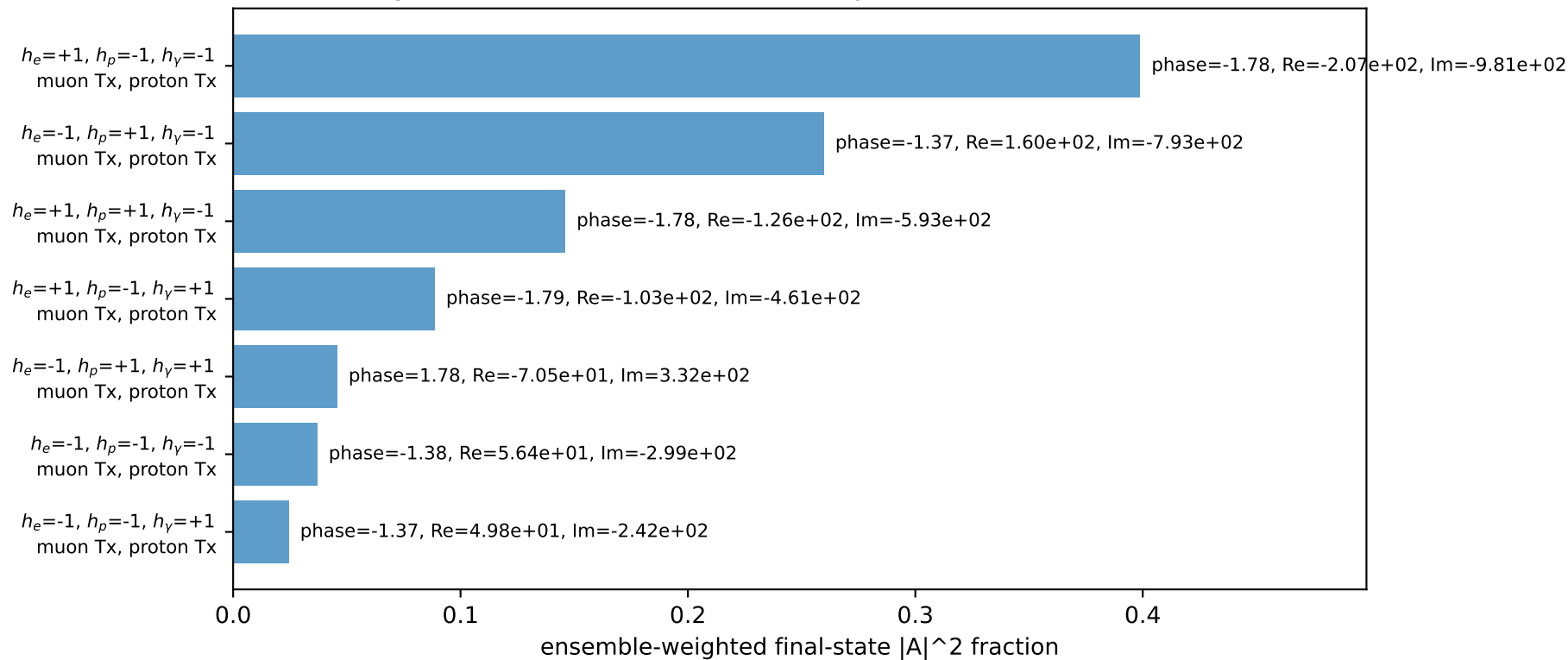
Leading initial-ensemble/final-state components (N=7, retained=99.9%)
