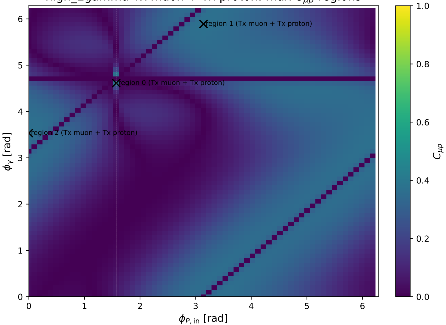
high_Egamma Tx muon + Tx proton: max C_{\mu p} regions
