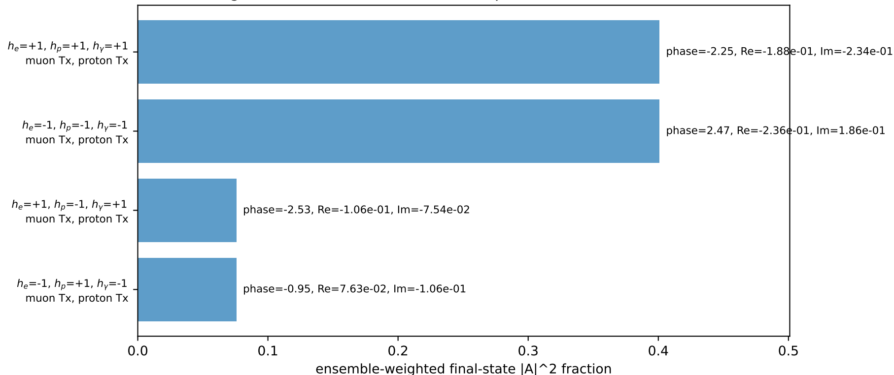
Leading initial-ensemble/final-state components (N=4, retained=95.3%)
