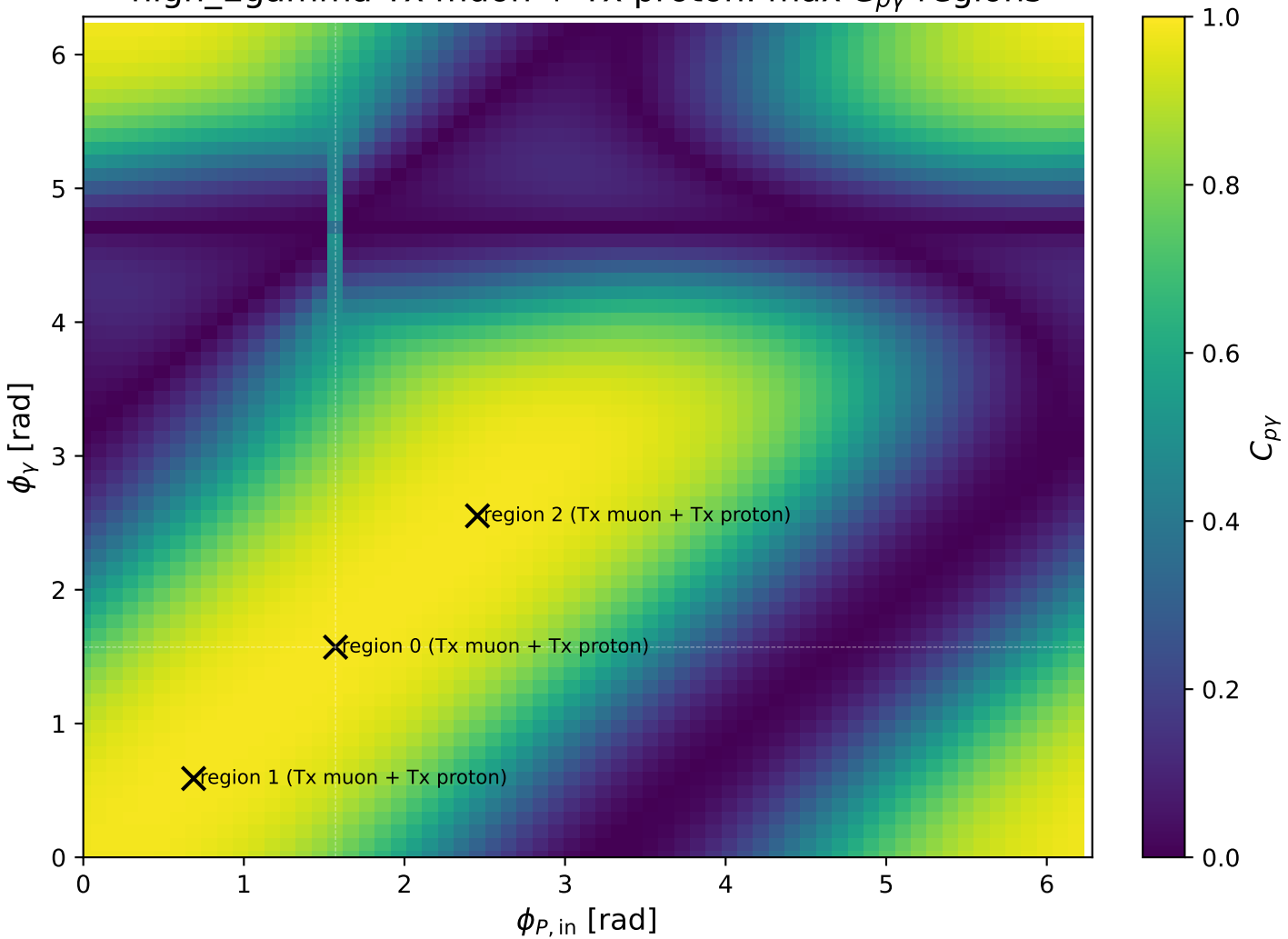
high_Egamma Tx muon + Tx proton: max C_{p\gamma} regions
